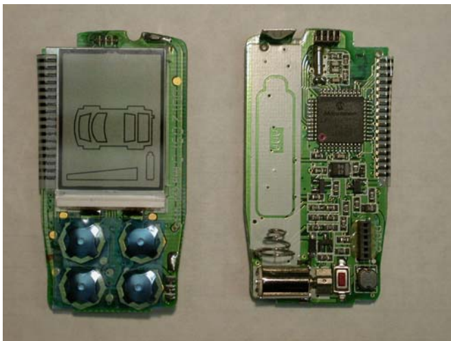
Photo 8 Main PCB top and bottom
