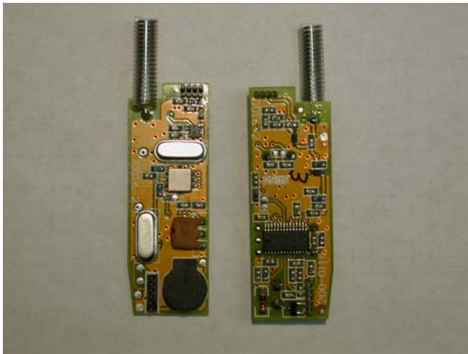
Photo 9 RF daughterboard PCB top and bottom
