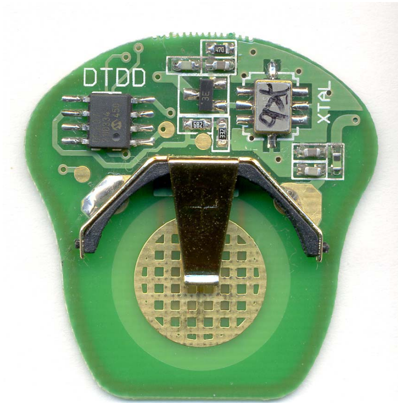
TRANSMITTER FRONT
