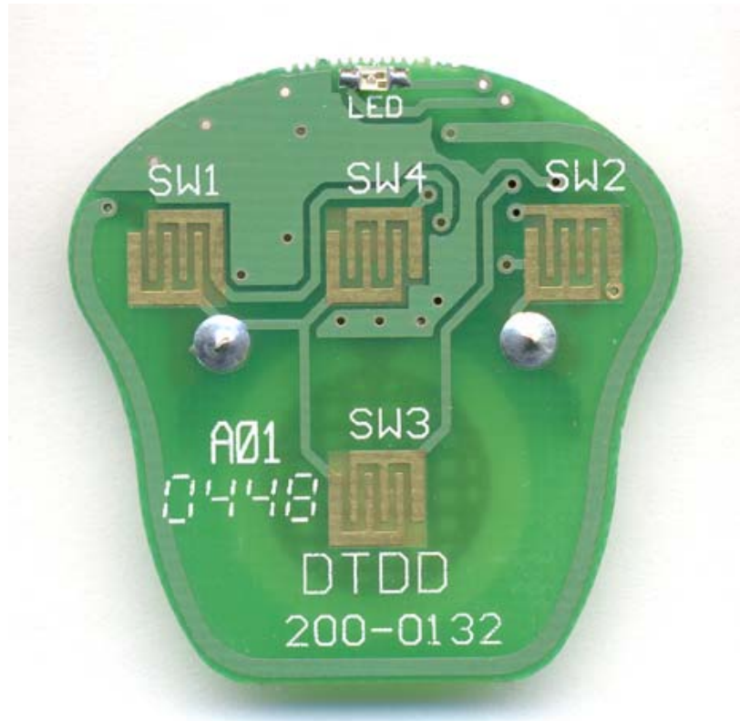
TRANSMITTER BACK
