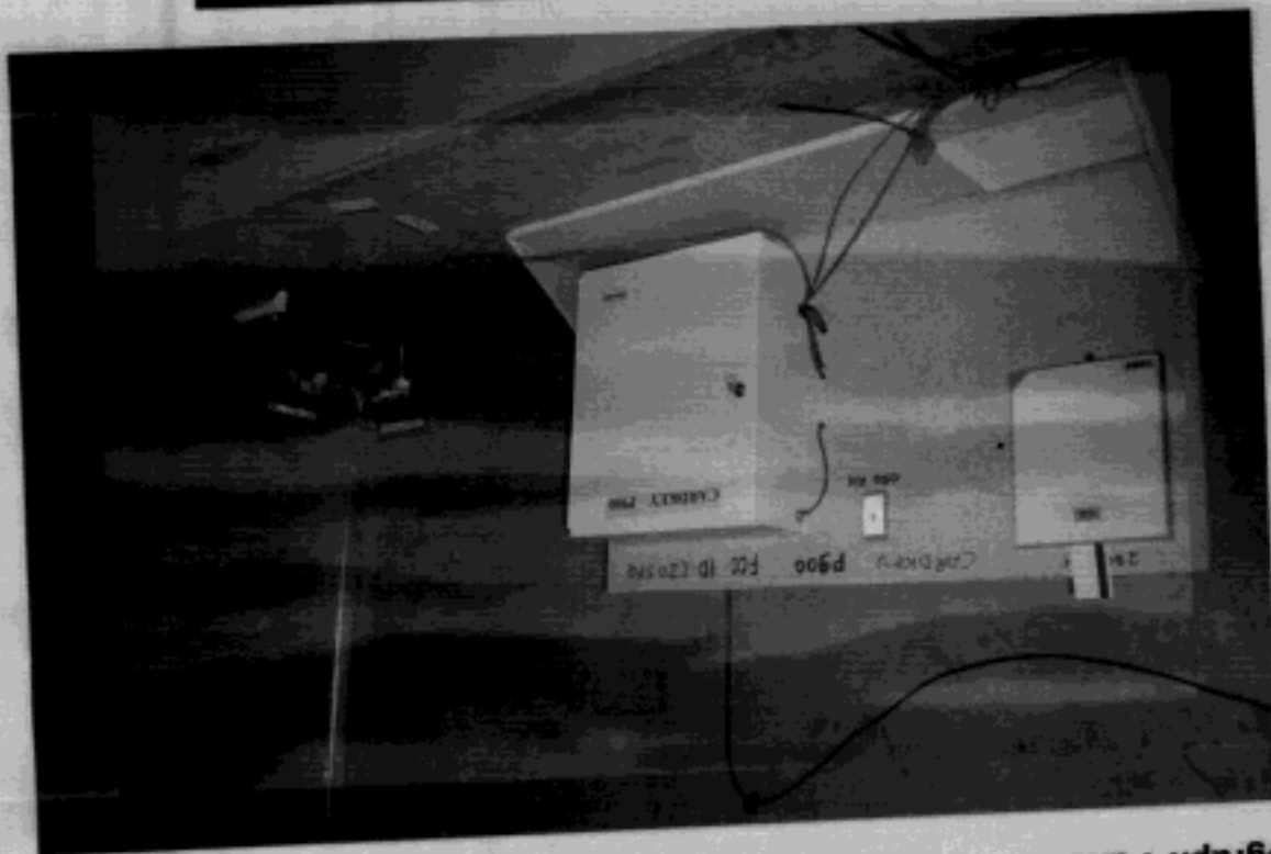
Photograph 1 and 2: Conducted Emissions Test Arrangement
