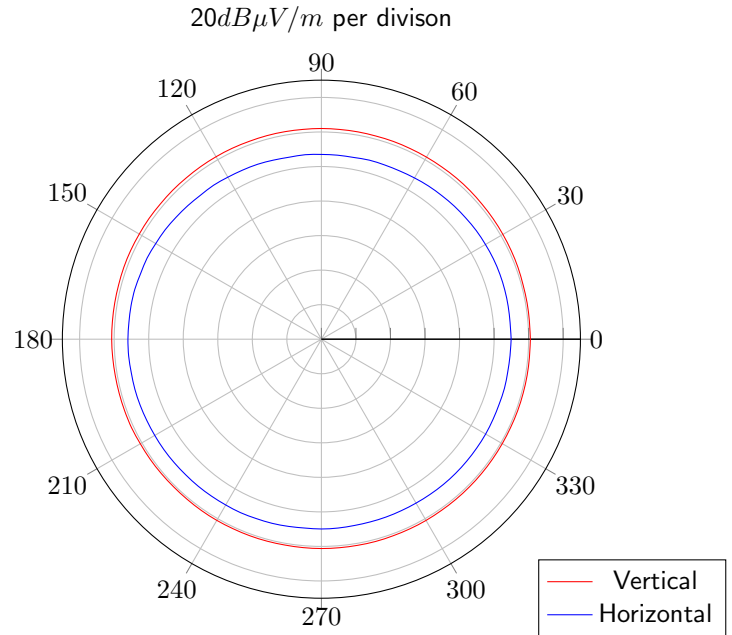
Figure 2: Radiation Pattern
