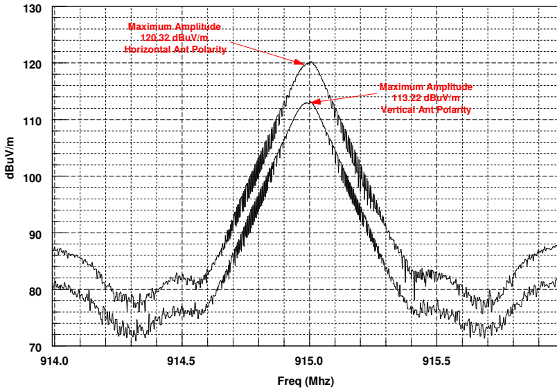
I TRON, Inc. Commercial Unit Model: 500S AM OOK 24 dBm Maximum Amplitude FCC 15.247 (b) (2) and RSS 247 5.4 (1) Middle Frequency
