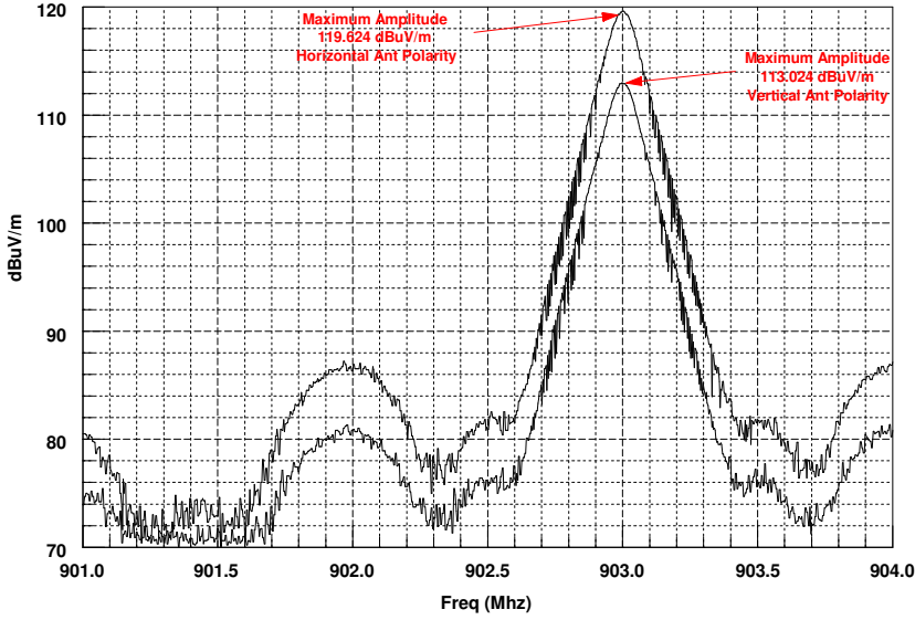
I TRON, Inc. Commercial Unit Model: 500S AM OOK 24 dBm Maximum Amplitude FCC 15.247 (b) (2) and RSS 247 5.4 (1) Low Frequency
