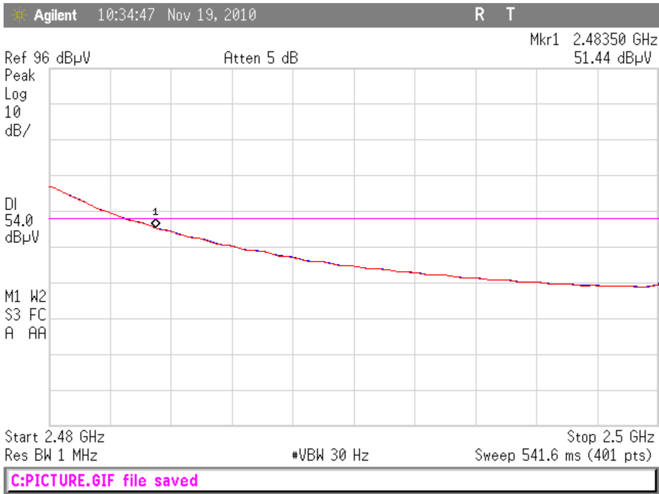
Figure 16: Average Horizontal Radiated Band Edge (2475MHz Fundamental)
