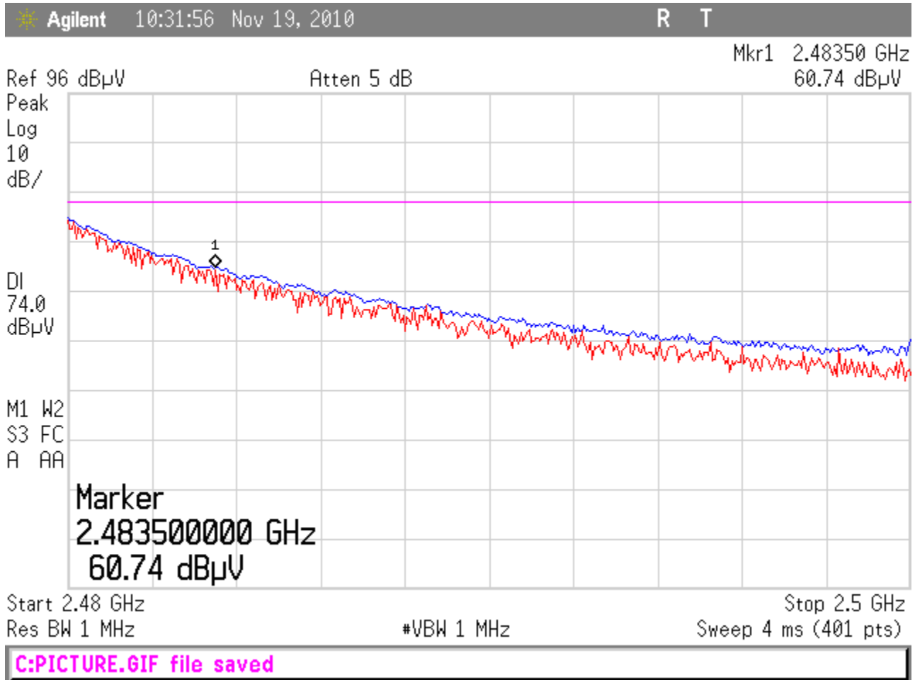
Figure 15: Peak Horizontal Radiated Band Edge (2475MHz Fundamental)
