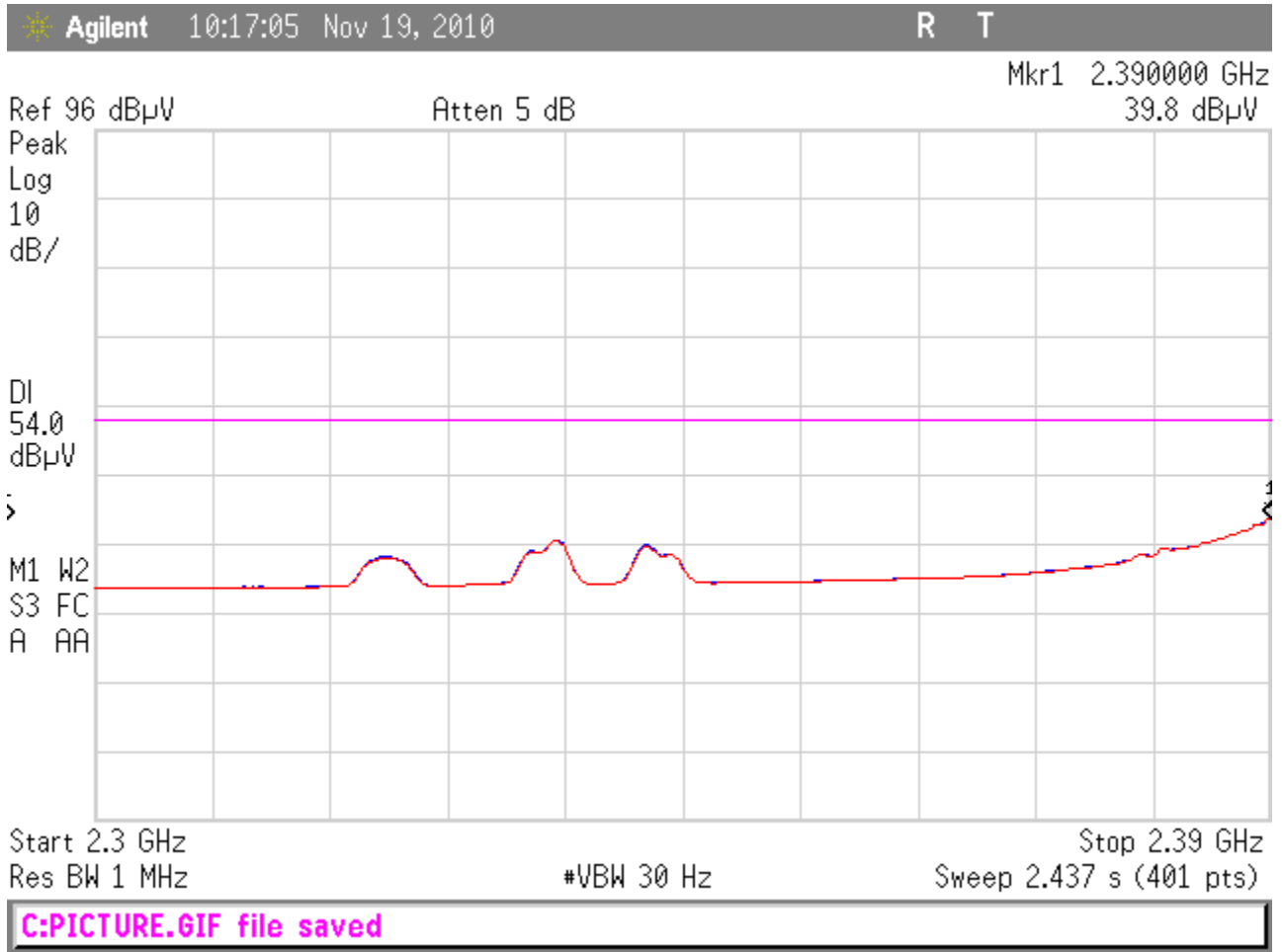
Figure 20: Average Horizontal Radiated Band Edge (2405MHz Fundamental)
