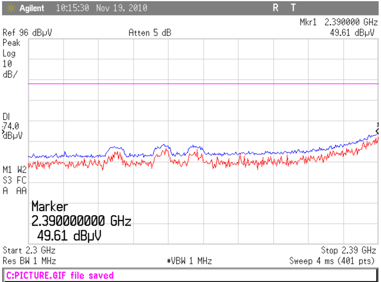
Figure 19: Peak Horizontal Radiated Band Edge (2405MHz Fundamental)
