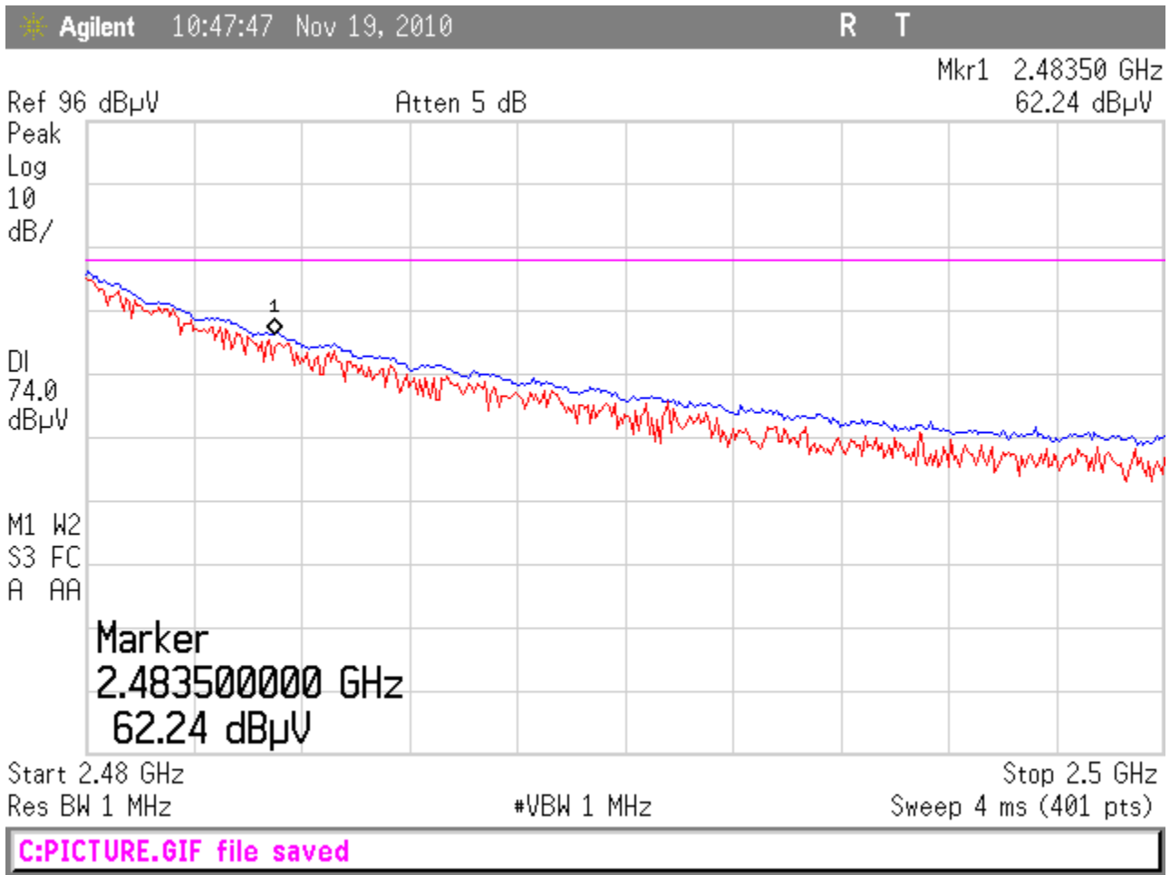
Figure 17: Peak Vertical Radiated Band Edge (2475MHz Fundamental)
