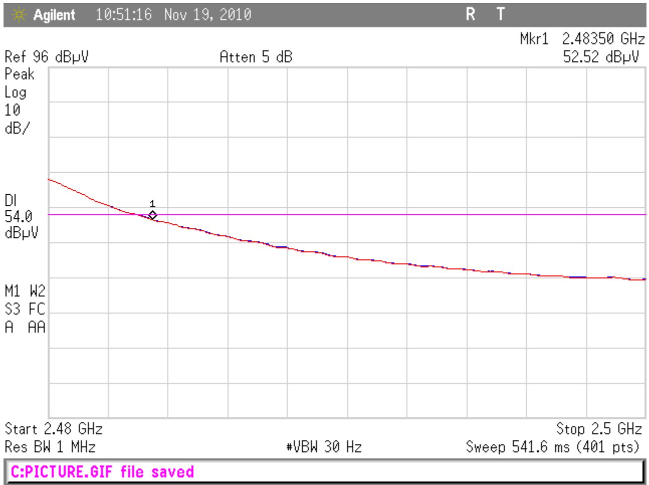
Figure 18: Average Vertical Radiated Band Edge (2475MHz Fundamental)
