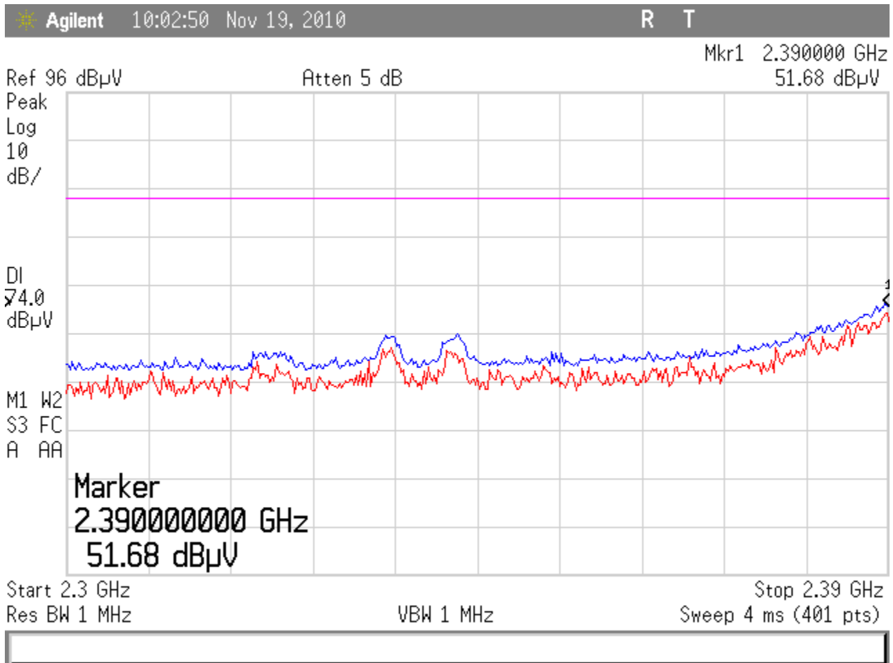
Figure 21: Peak Vertical Radiated Band Edge (2405MHz Fundamental)
