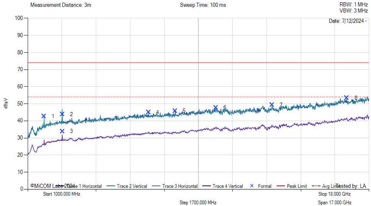
FCC Spurious 1 GHz -18 GHz
