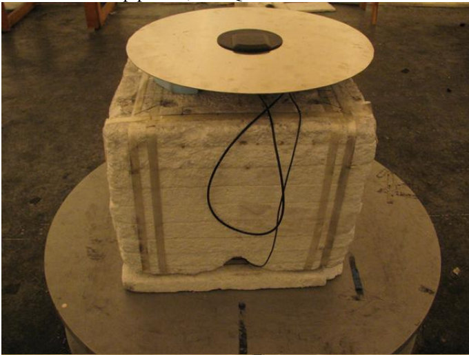
100WB test setup photos; EWQ100WB and 864D-100WB
