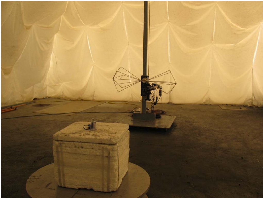
100W test setup photos; EWQ100W and 864D-100W
