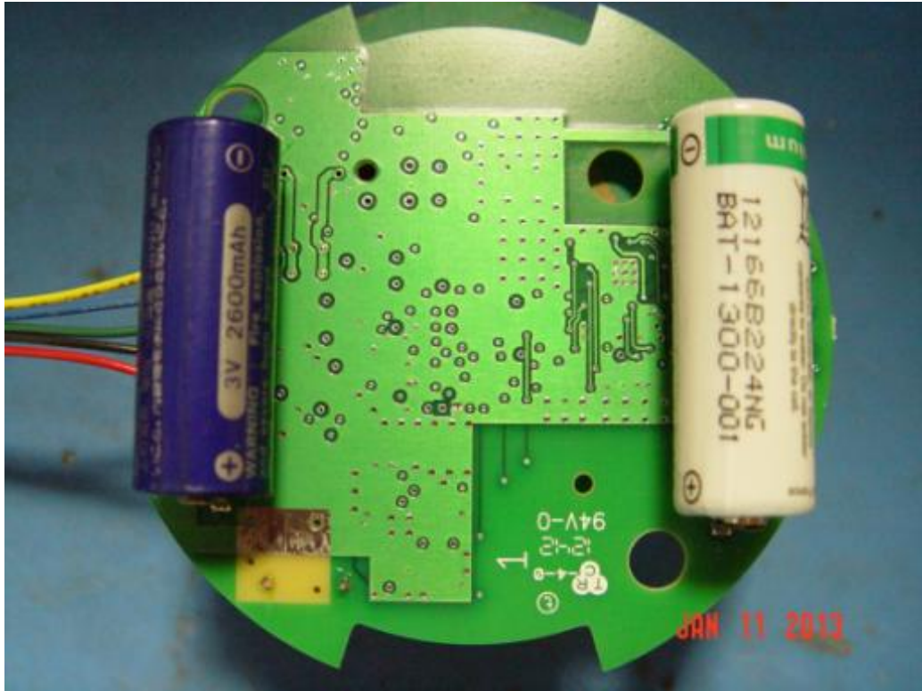
Printed circuit board assembly used in TEL-5013-001 Bottom Side.
