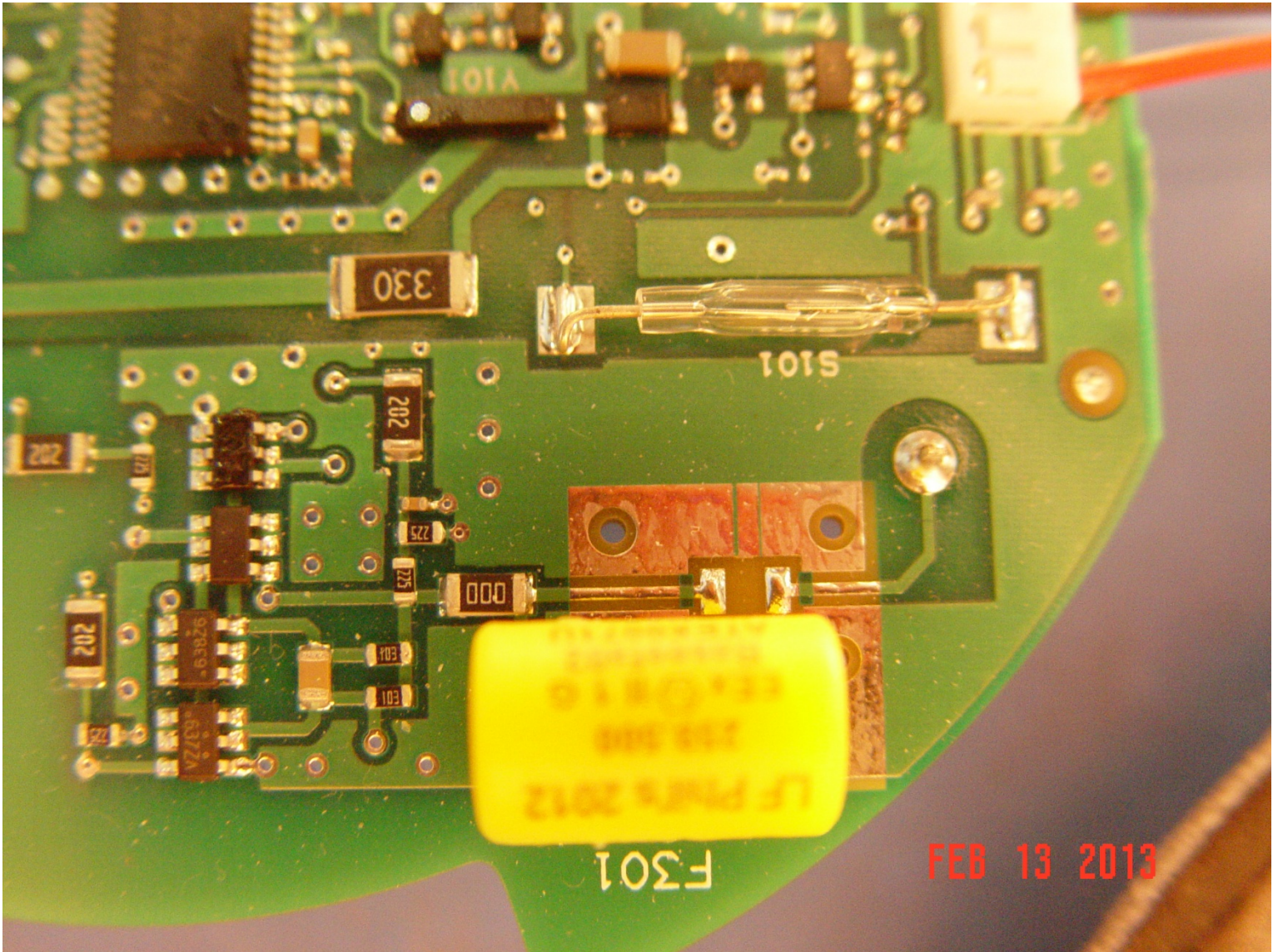
Printed circuit board assembly used in TEL-5013-001 Top Side (power supply area).
