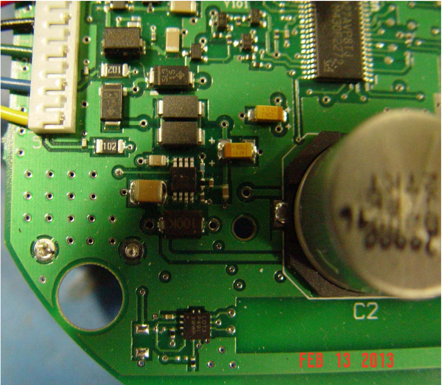
Printed circuit board assembly used in TEL-5013-001 Top Side (interface area).
