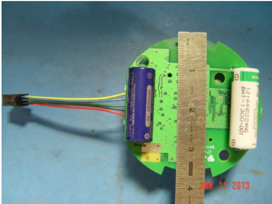
Printed circuit board assembly used in TEL-5013-001 width view.
