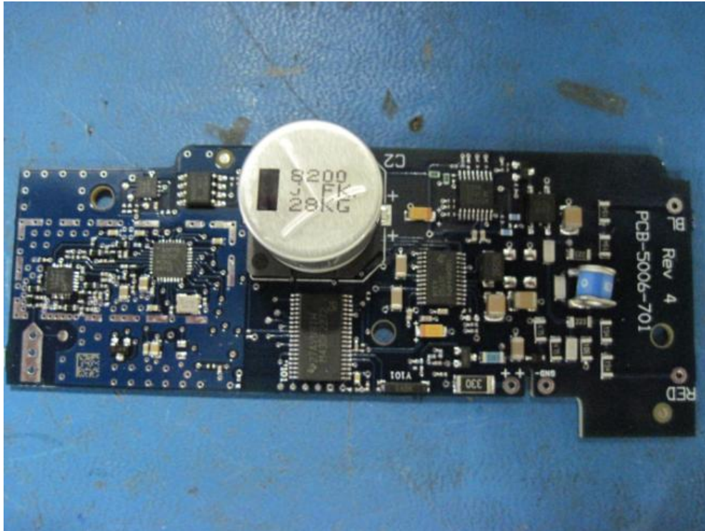
Printed circuit board assembly used in TEL-1000-003 Top Side.
