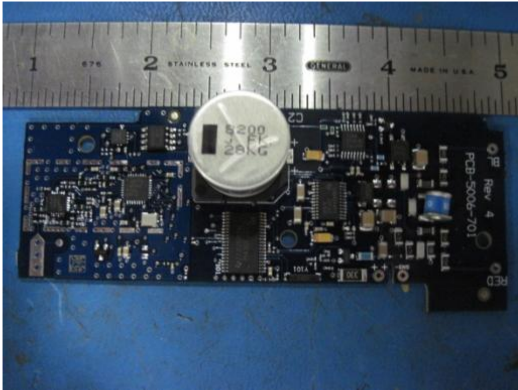
Printed circuit board assembly used in TEL-1000-003 height view.
