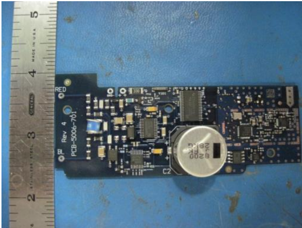
Printed circuit board assembly used in TEL-1000-003 width view.
