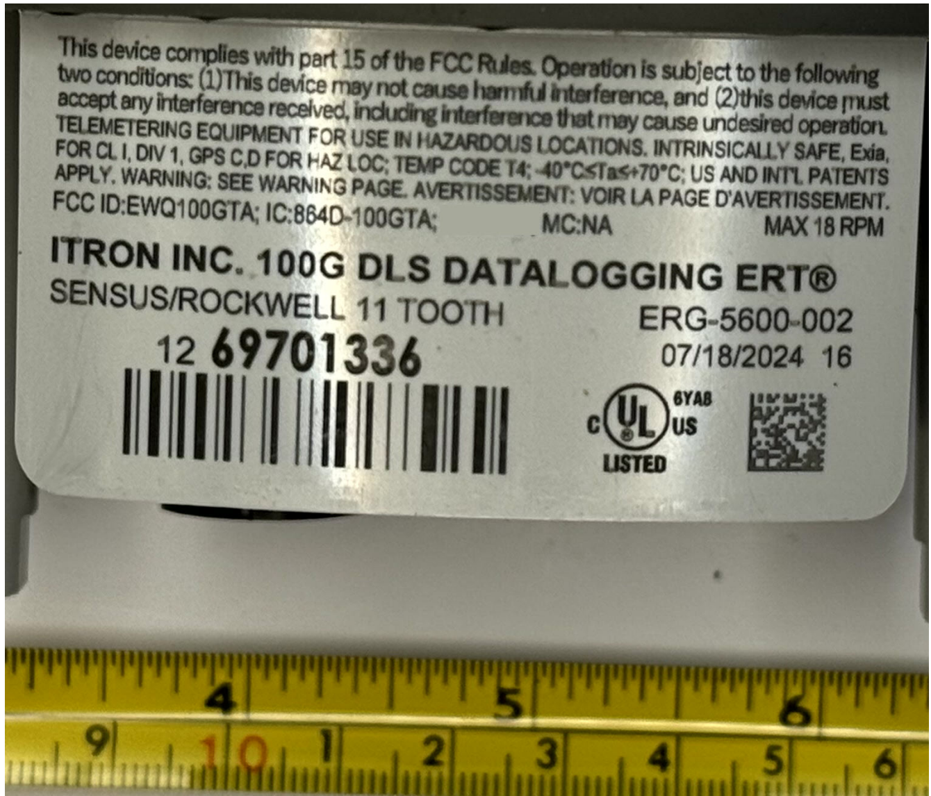
Figure 3.1: ERG-5600-002 Label
