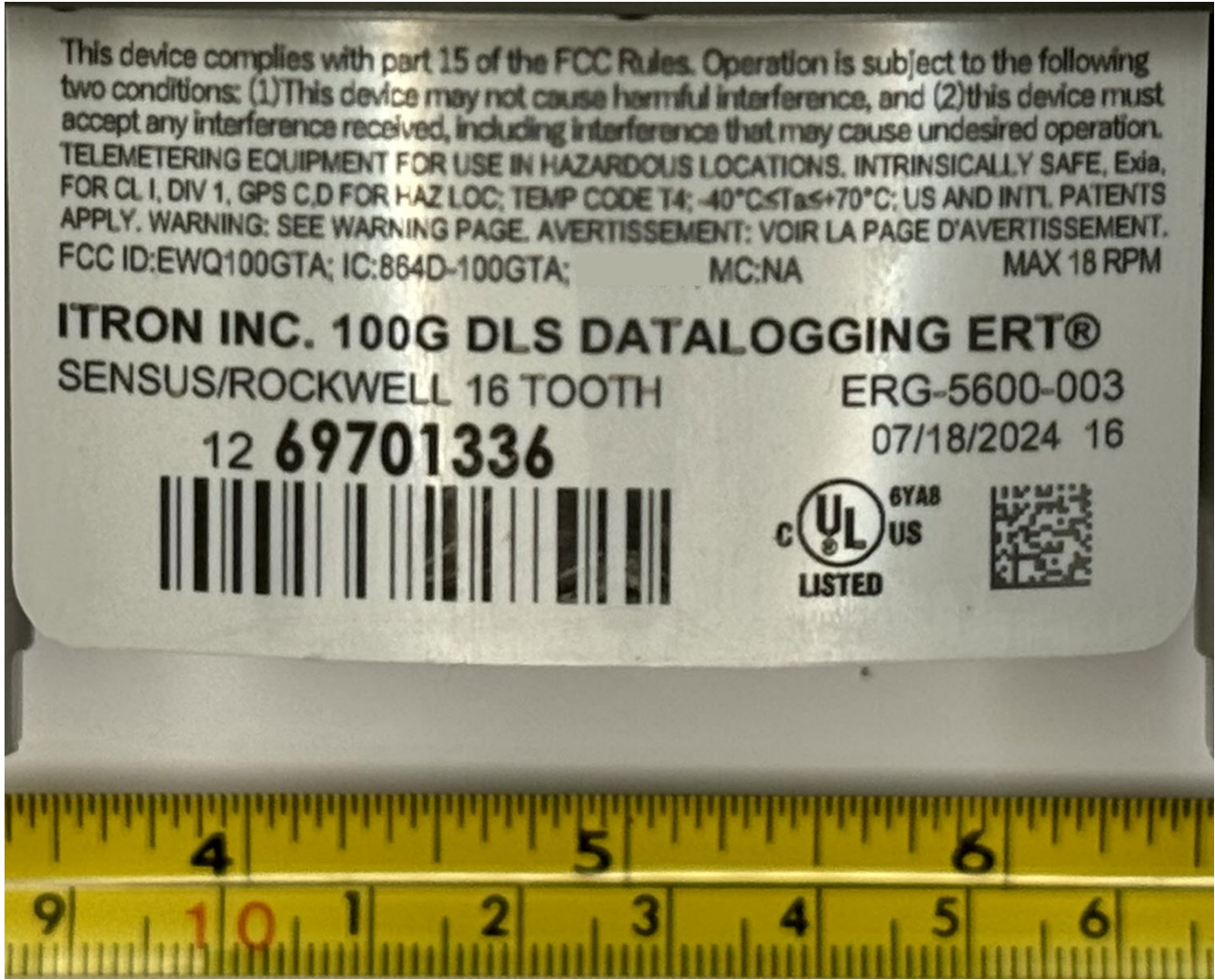
Figure 4.1: ERG-5600-003 Label
