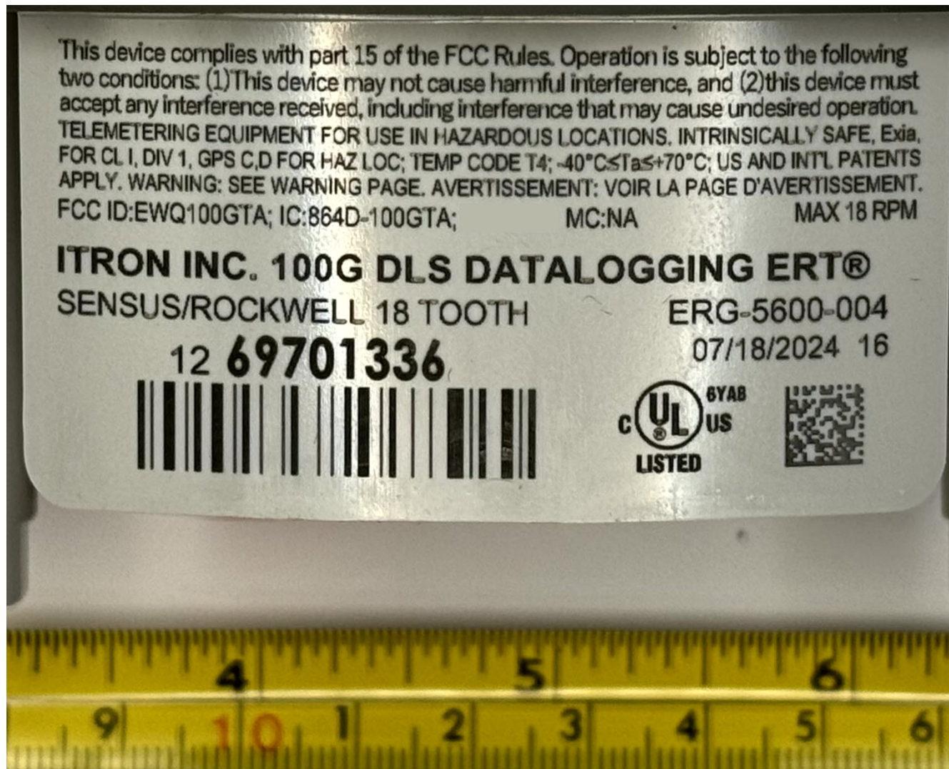
Figure 5.1: ERG-5600-004 Label
