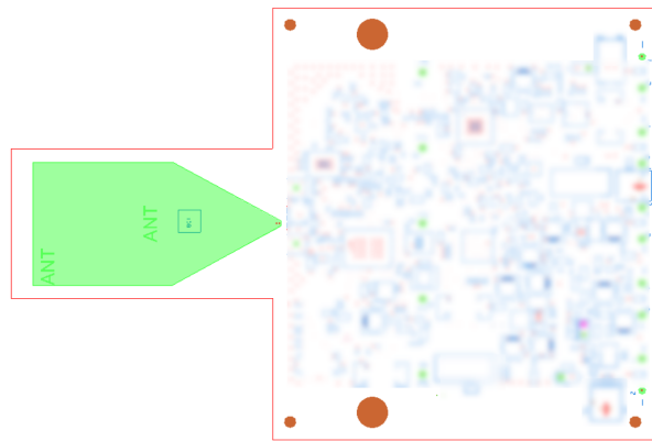
Figure 1: Antenna Structure
