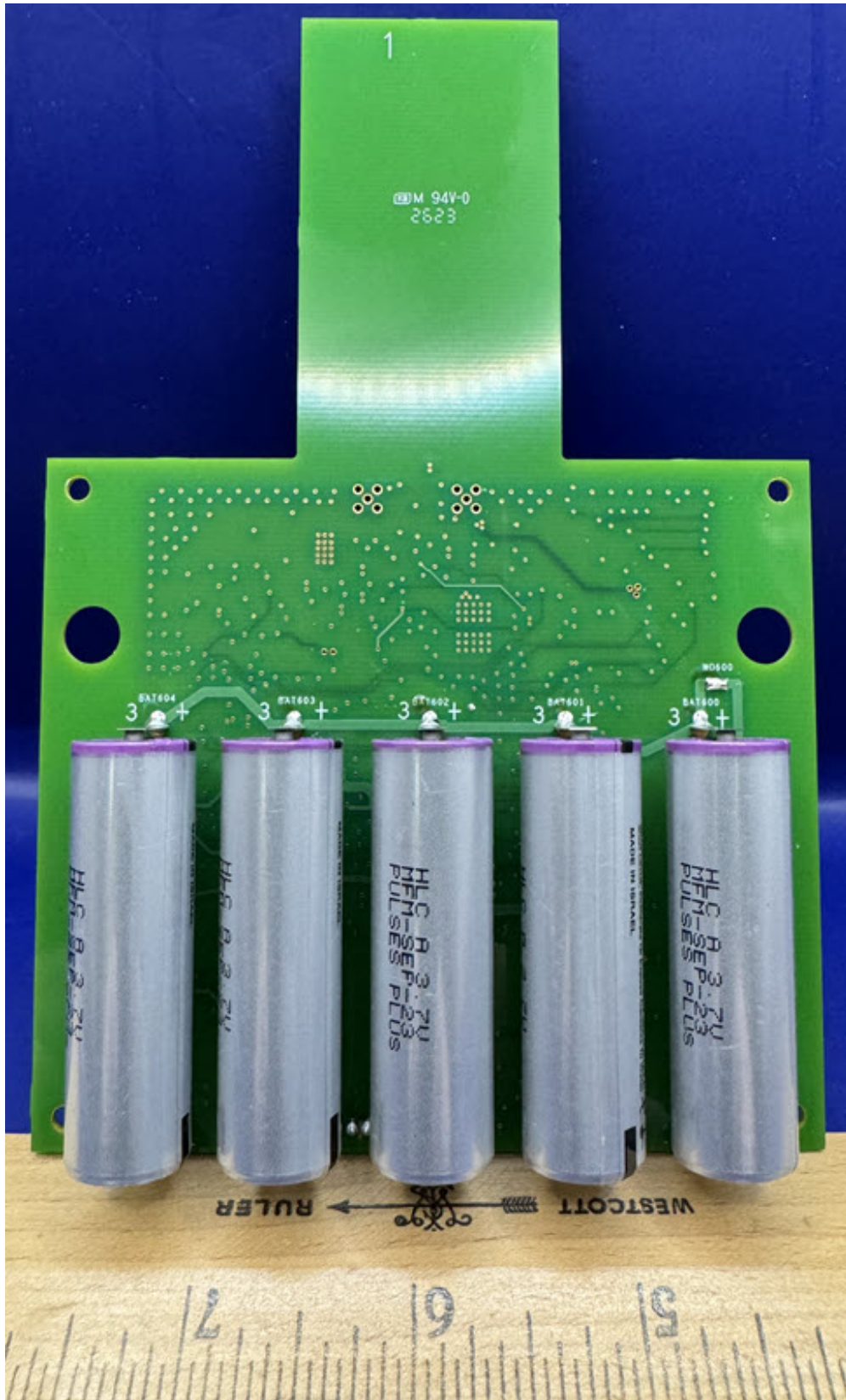
Figure 1.2: PCB Back
