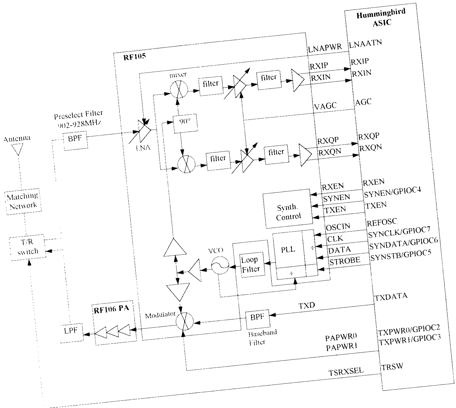
RF Transceiver (RF105 & RF106) Block Diagram
