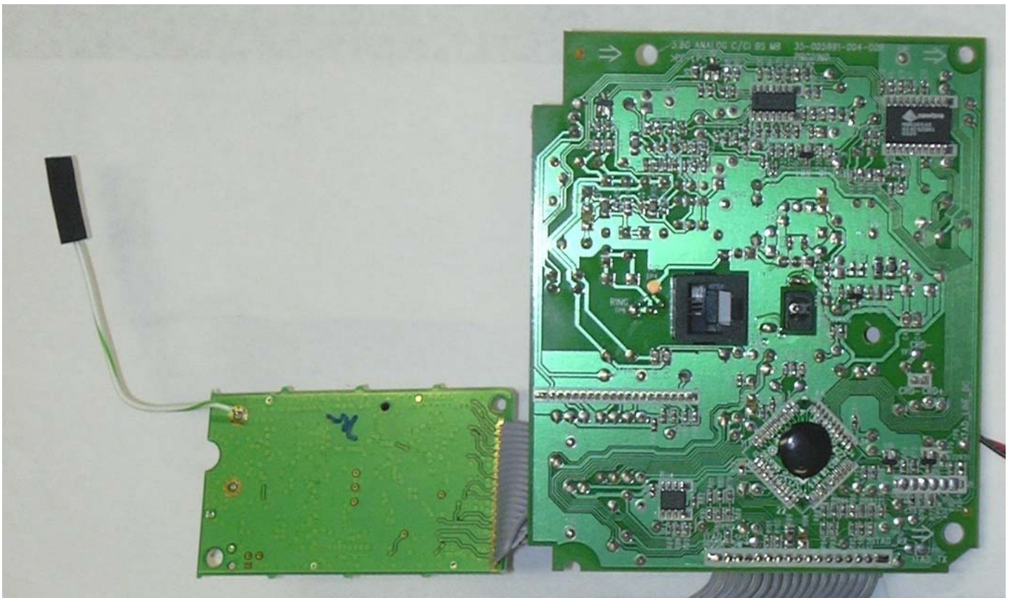
VTech ia5854 - with New Base RF Antennas
