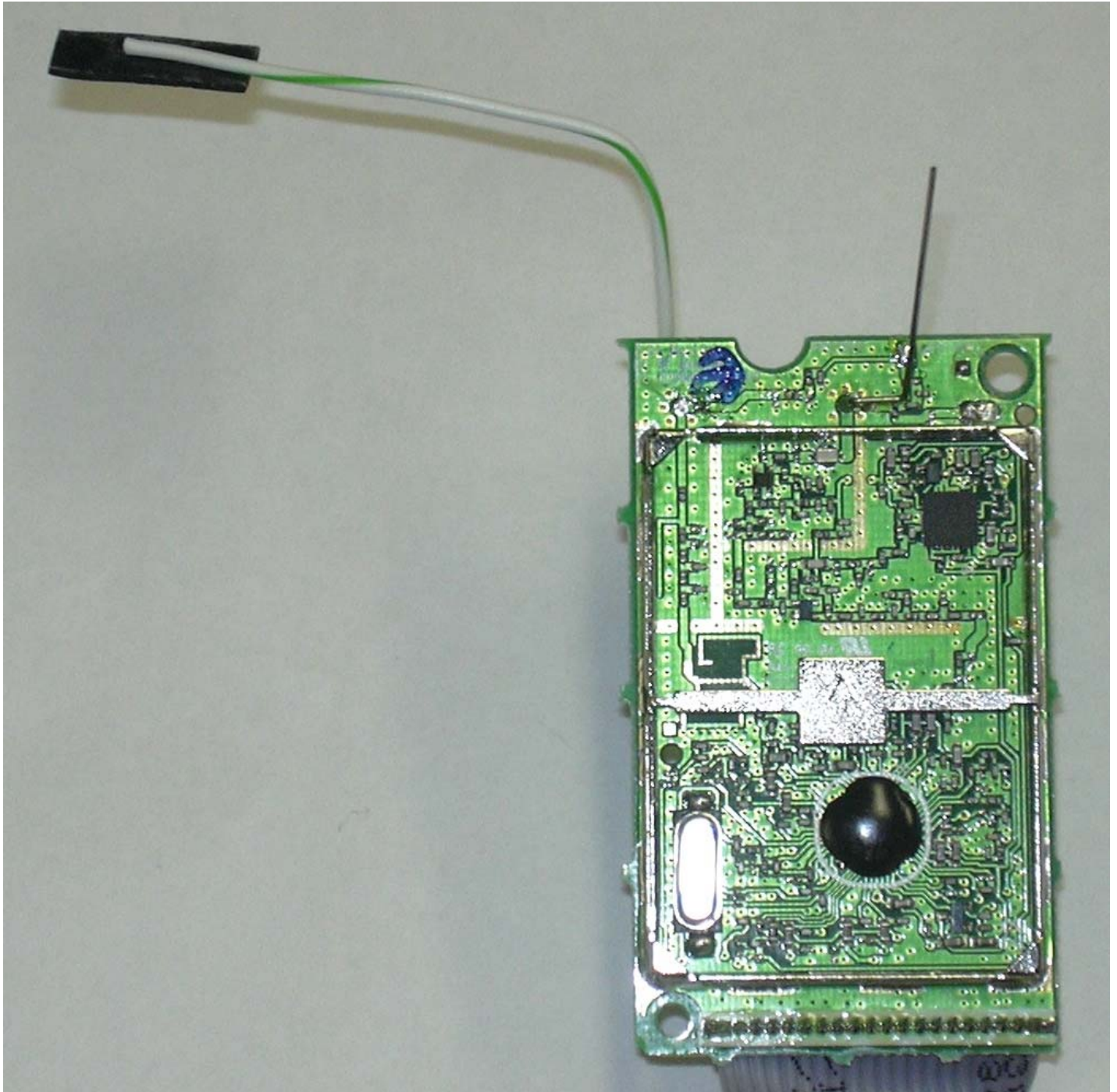
VTech ia5854 - with New Base RF Antennas
