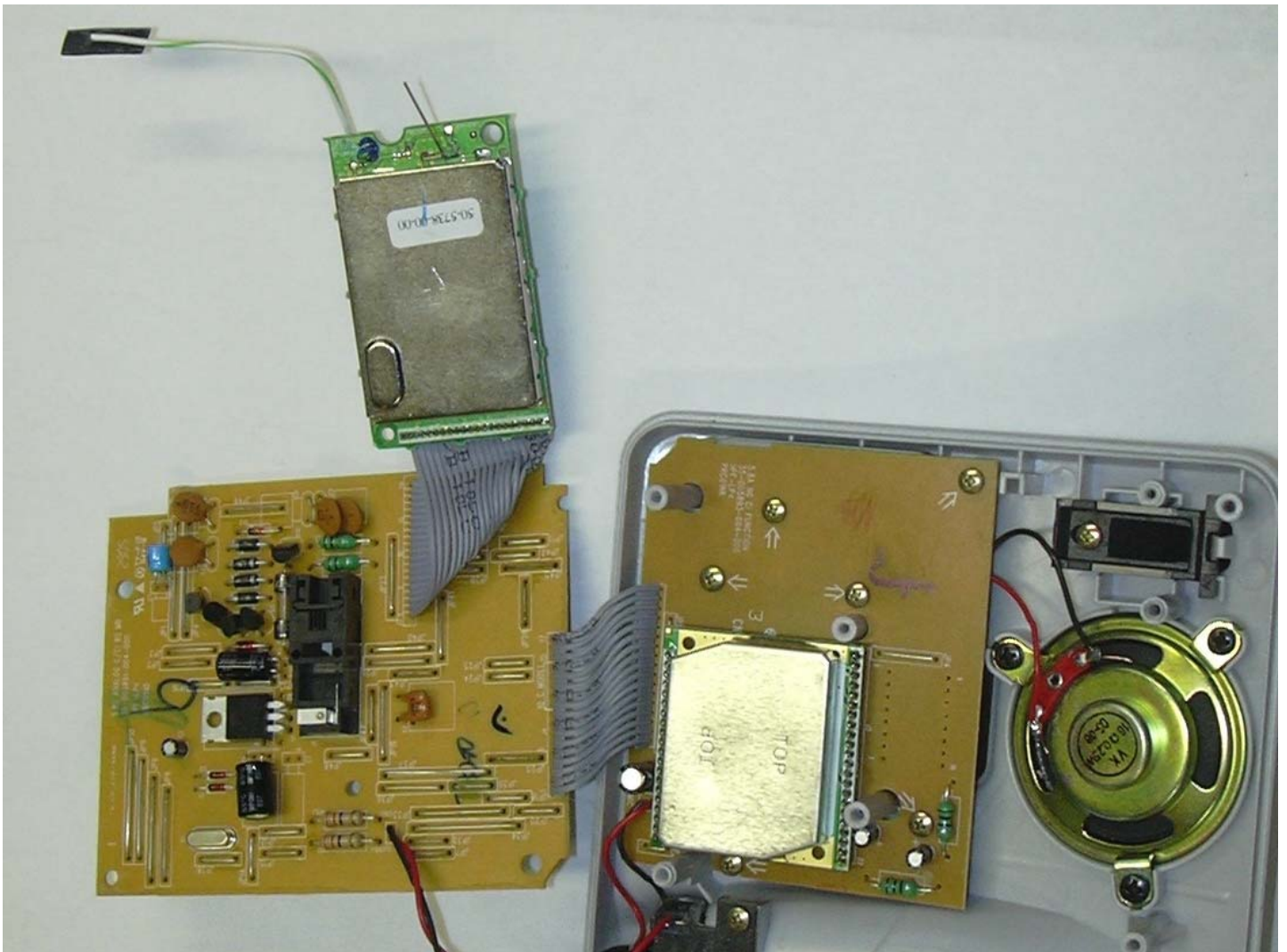
VTech ia5854 - with New Base RF Antennas
