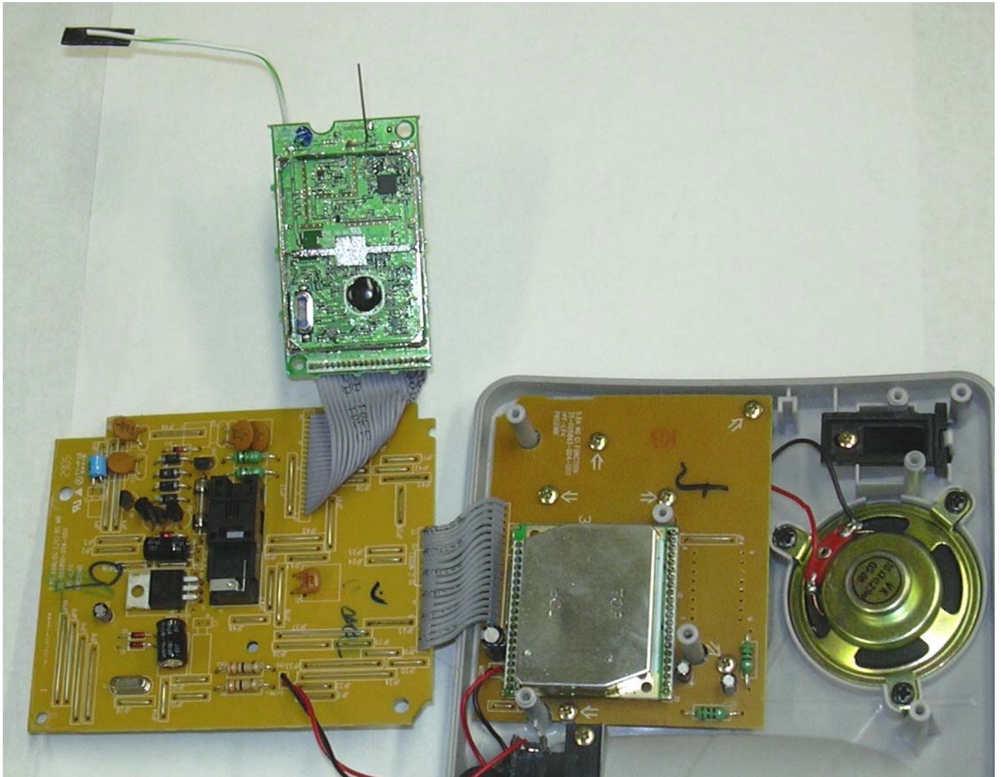
VTech ia5854 - with New Base RF Antennas
