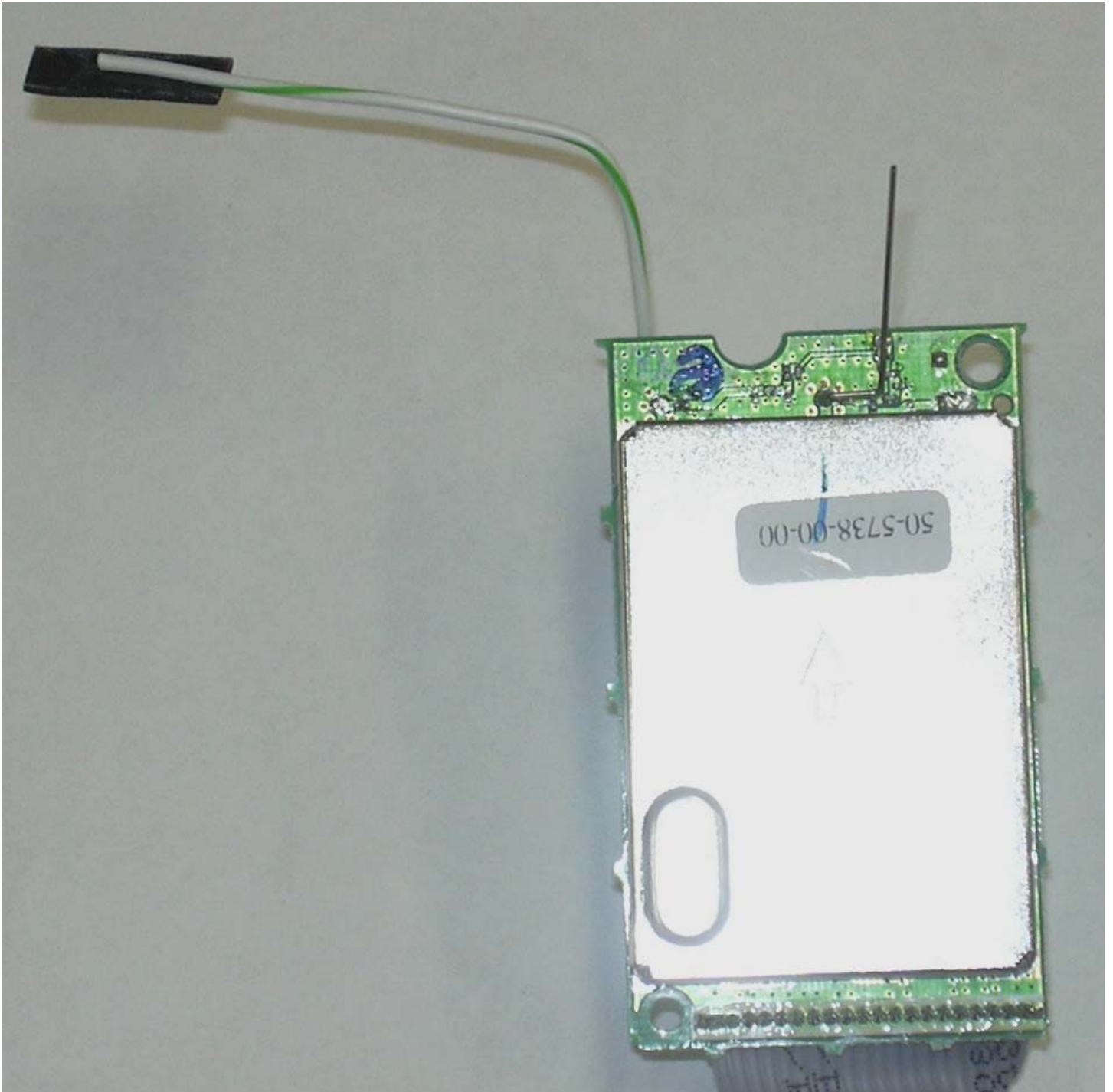
VTech ia5854 - with New Base RF Antennas
