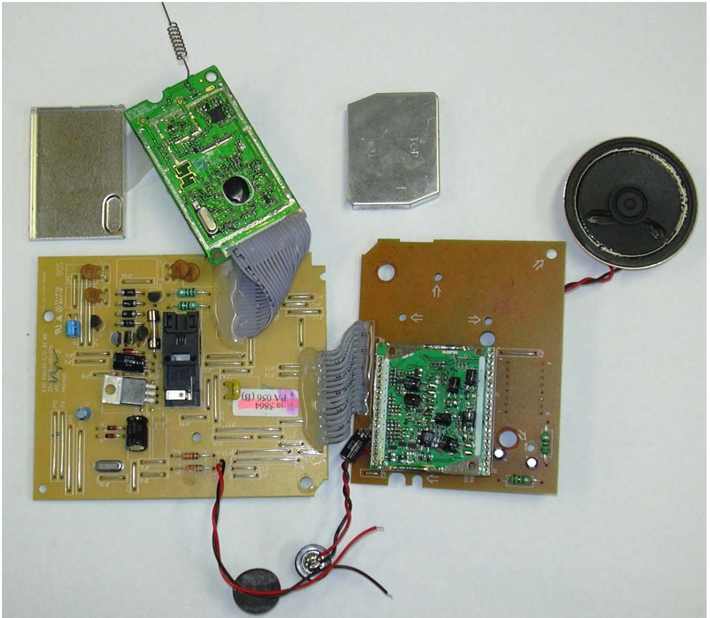
VTech ia5854 / ia5864 / ia5874 Base PCB
