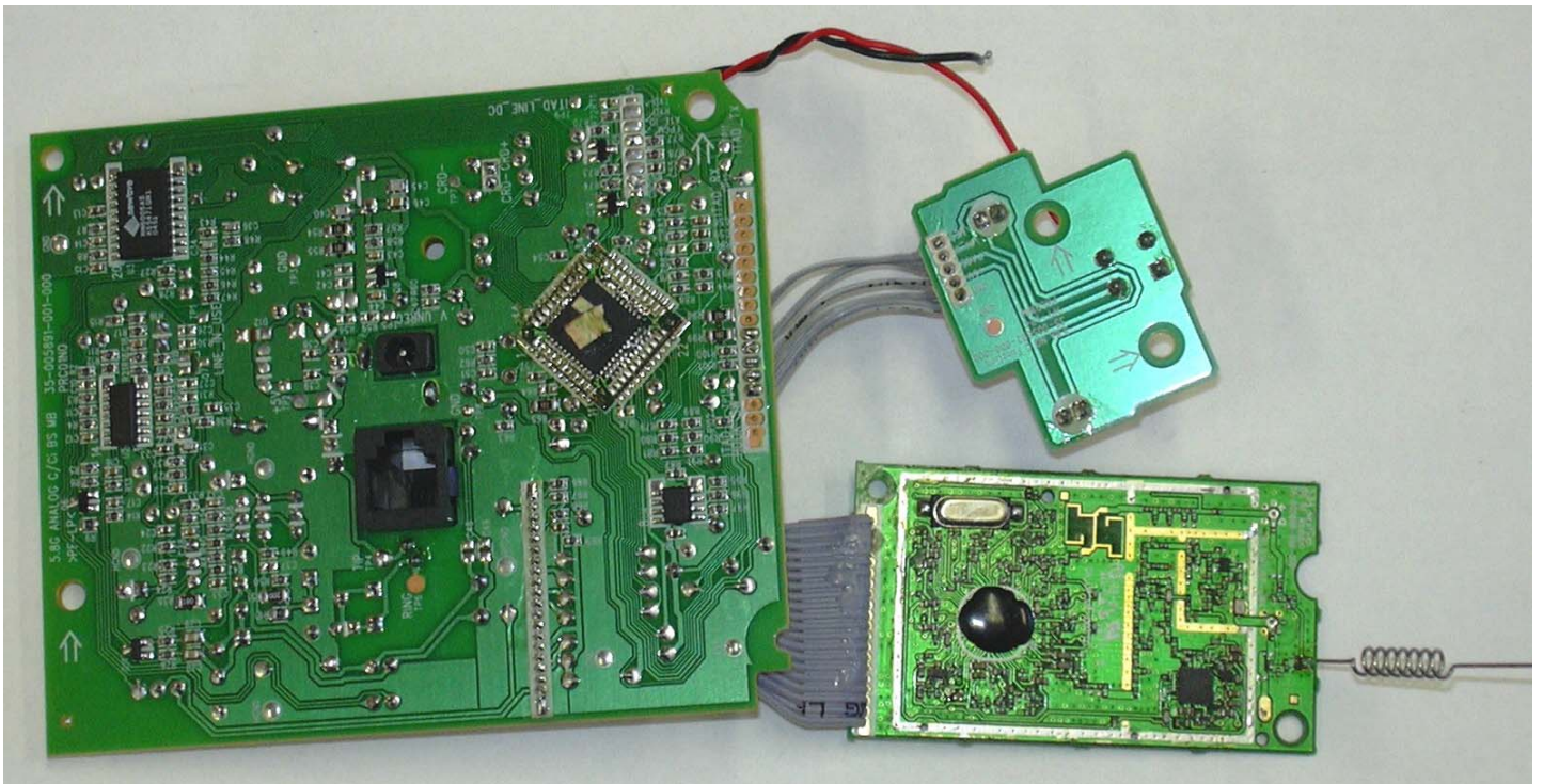
VTech ia5823_ia5845 Base PCB
