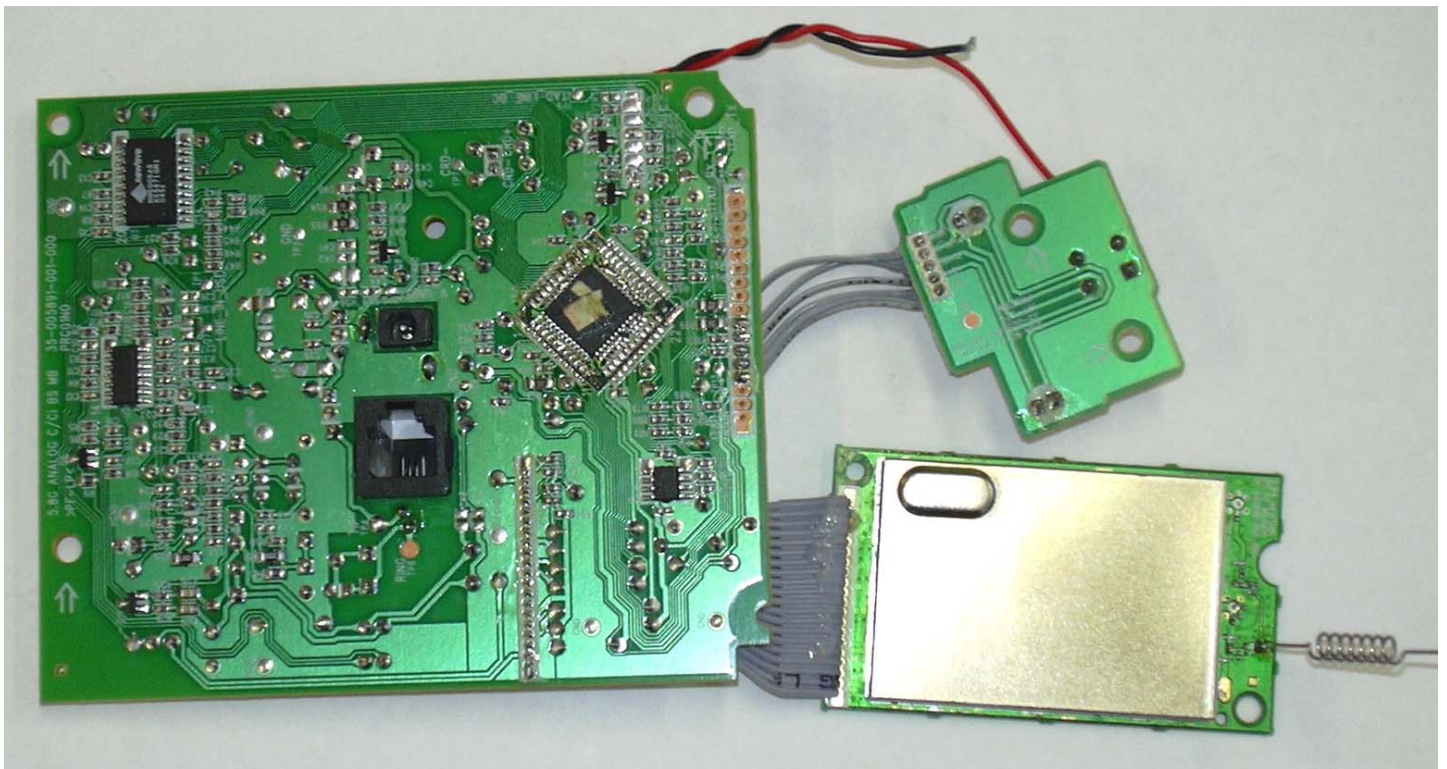
VTech ia5823_ia5845 Base PCB
