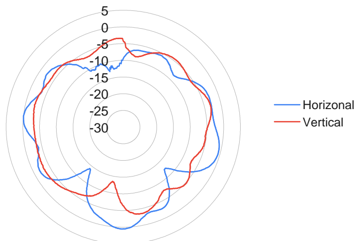
Antenna gain
