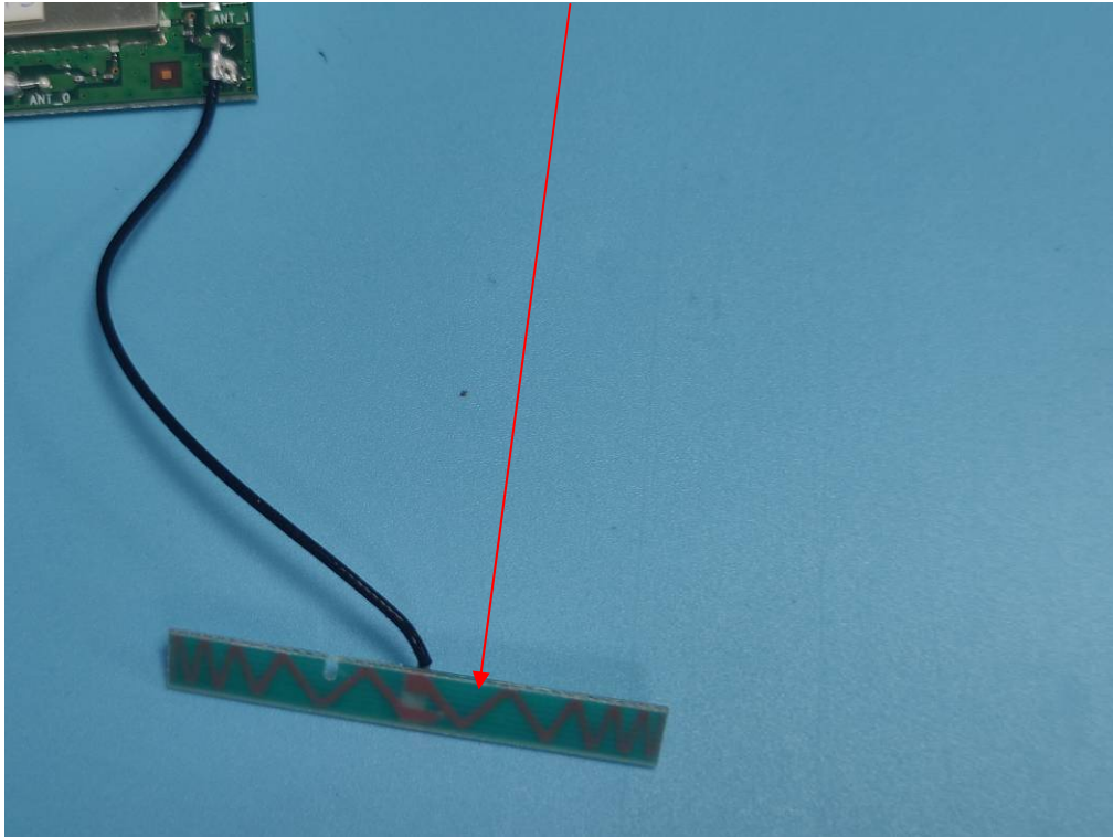
DECT ANT1
