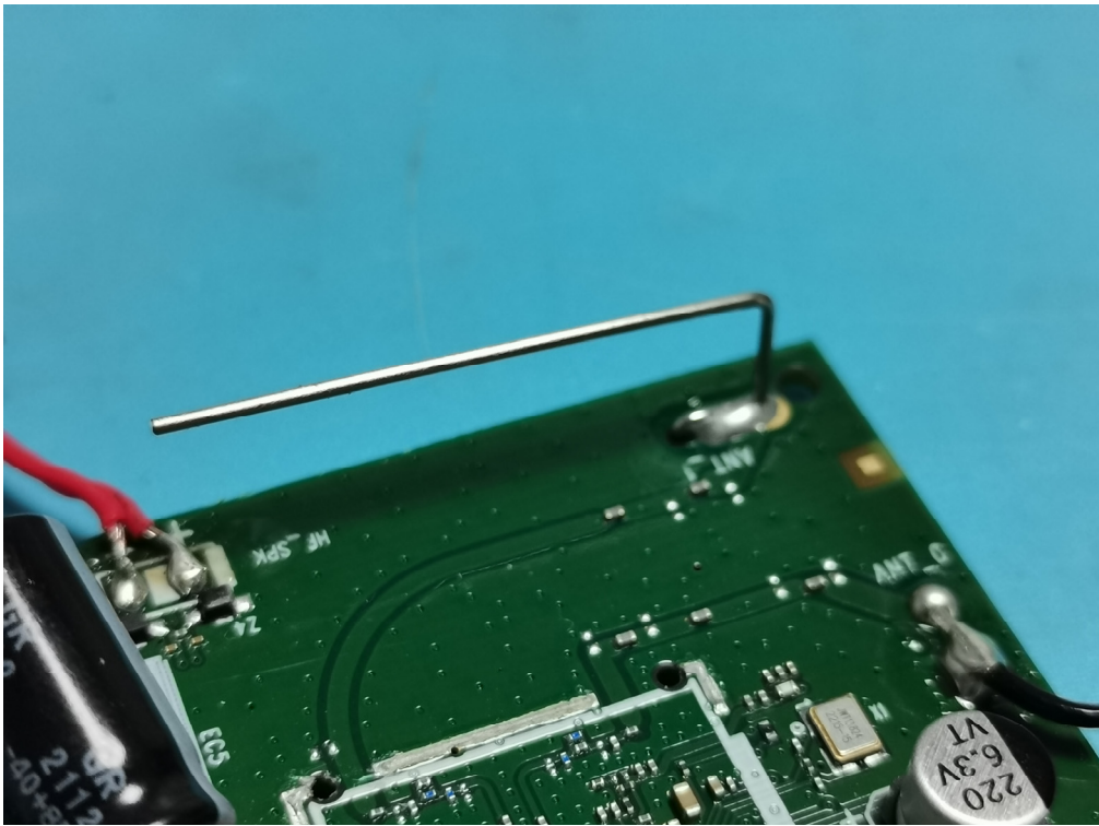
Antenna 0
