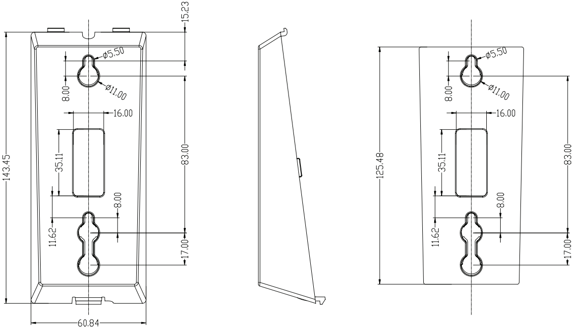
Single Drawing(Scale 1:1)
