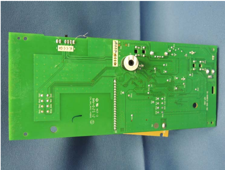
SIP Corded Deskset Main PCB solder side
