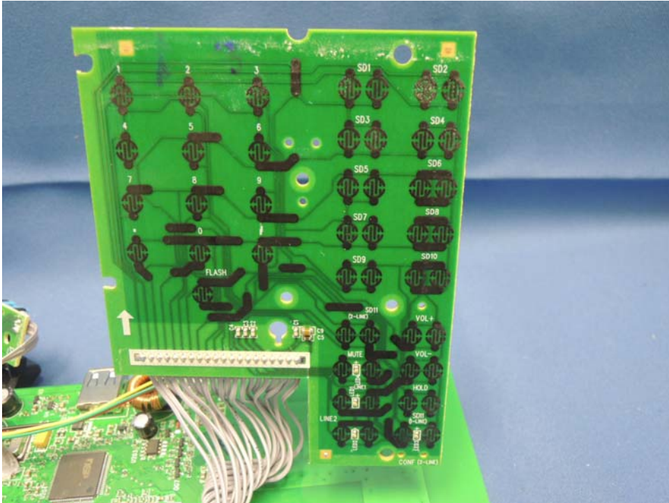
SIP Corded Deskset Keypad front side
