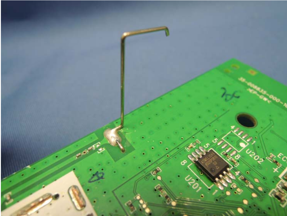
SIP Corded Deskset Antenna
