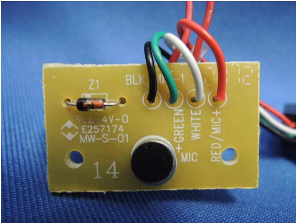
SIP Corded Deskset Mic.. Board front side
