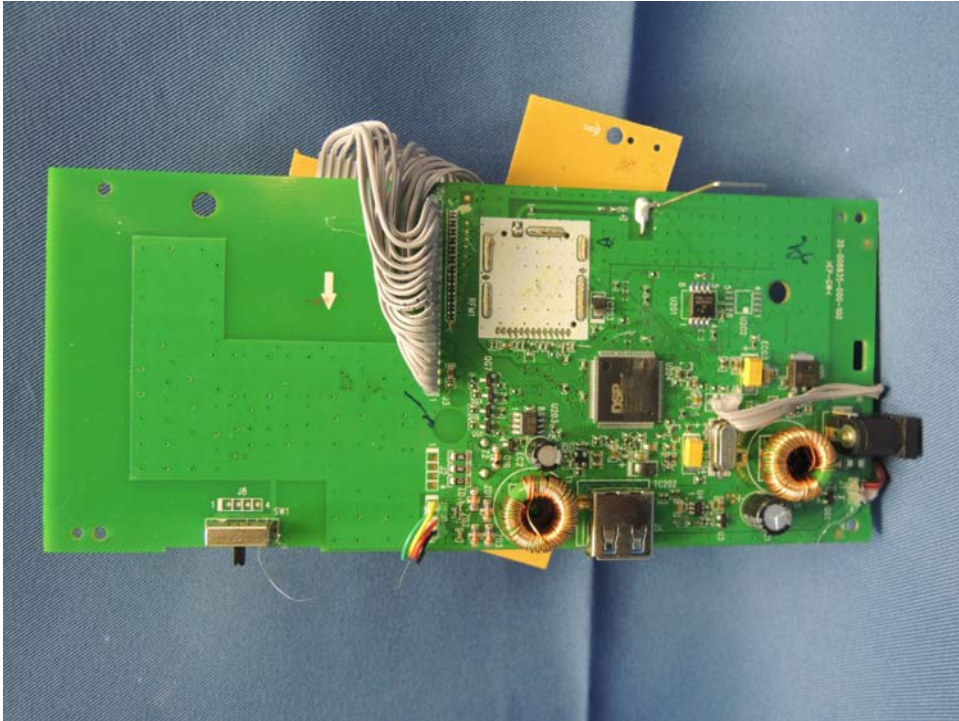
SIP Corded Deskset Main PCB comp side (View 2)
