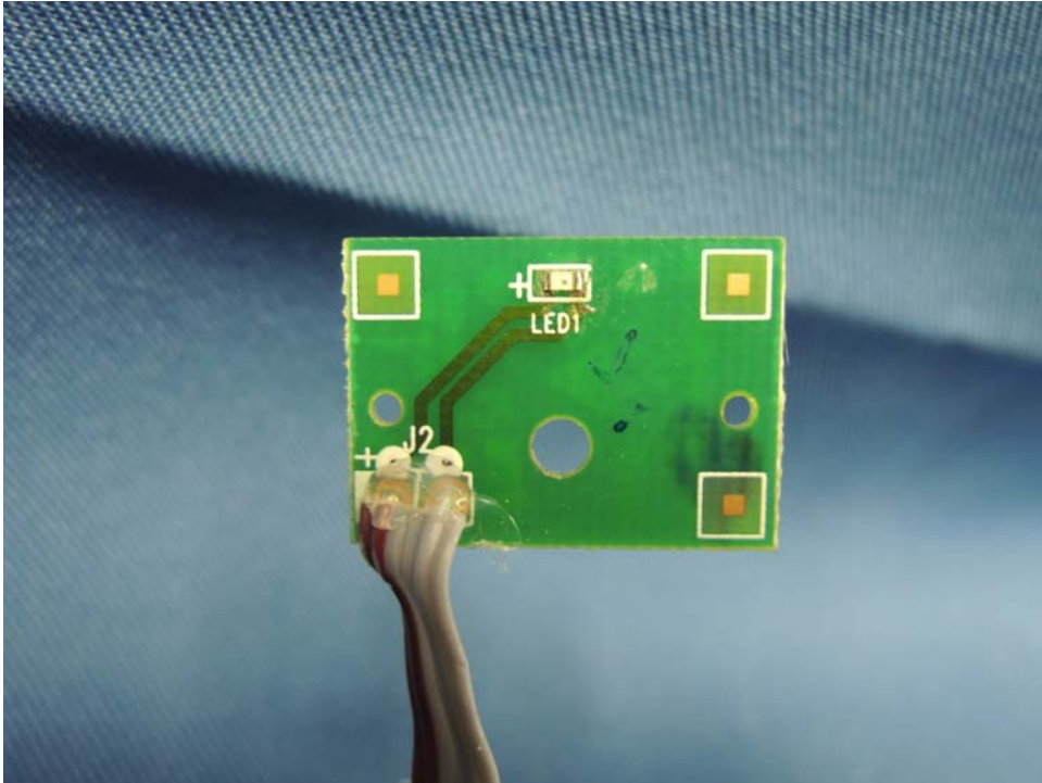
SIP Corded Deskset LED front side
