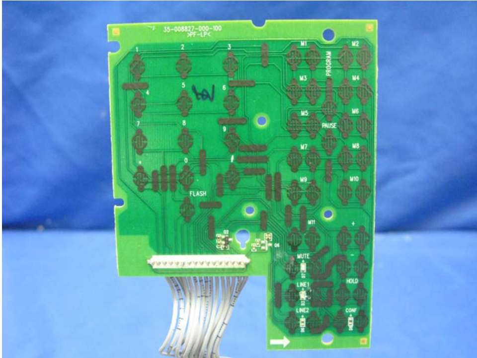
Deskset Keypad front side
