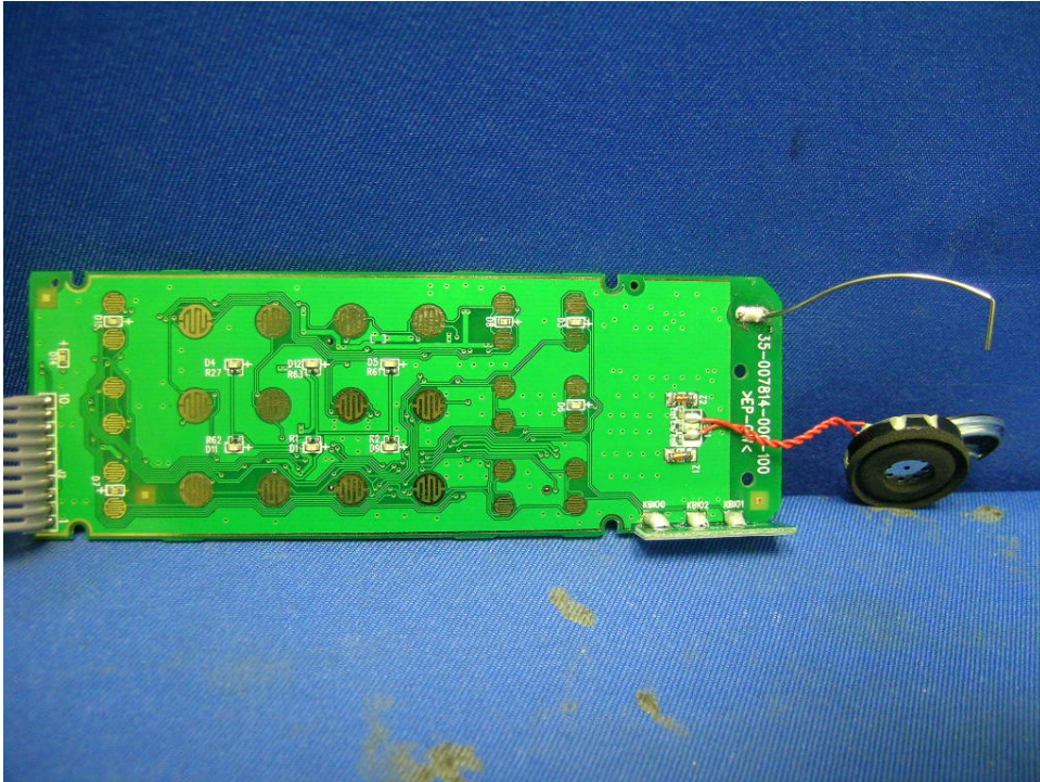
Handset PCB (View 1)
