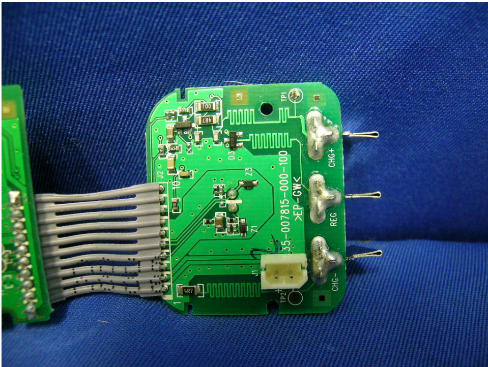
Handset PCB (View 2)
