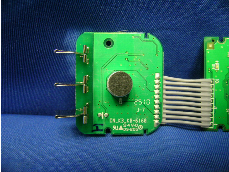
Handset PCB (View 3)
