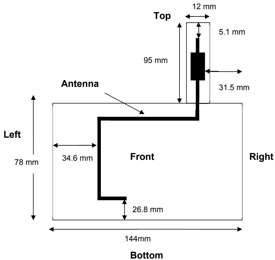
(Antenna Extended)
