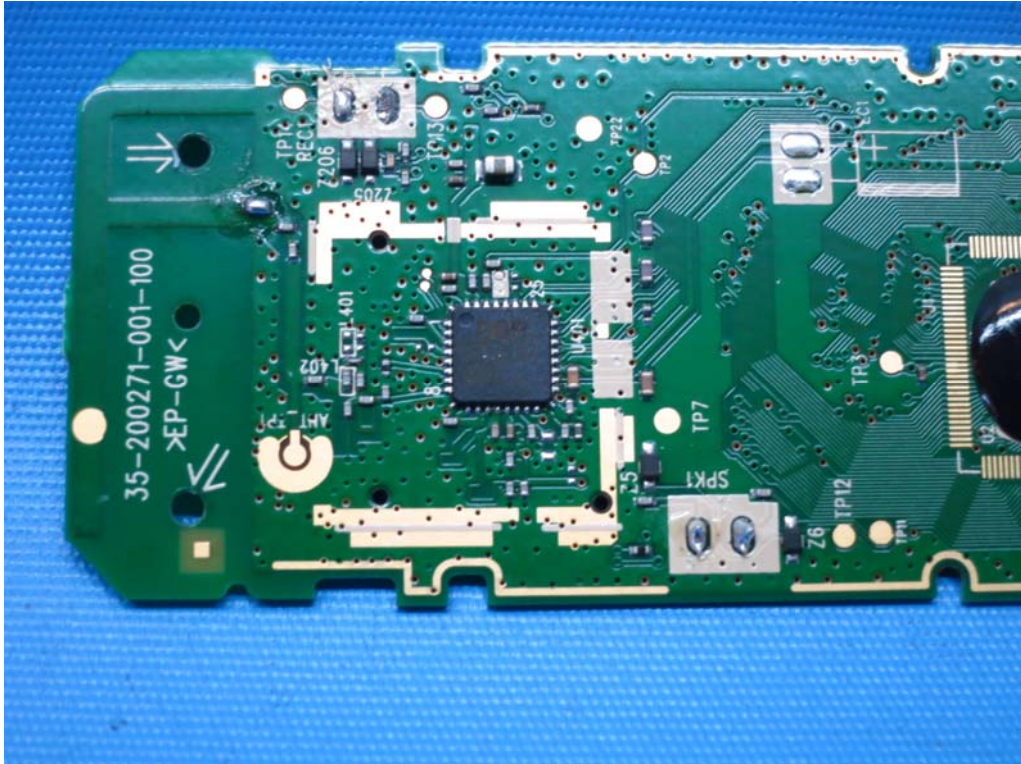
Handset Antenna
