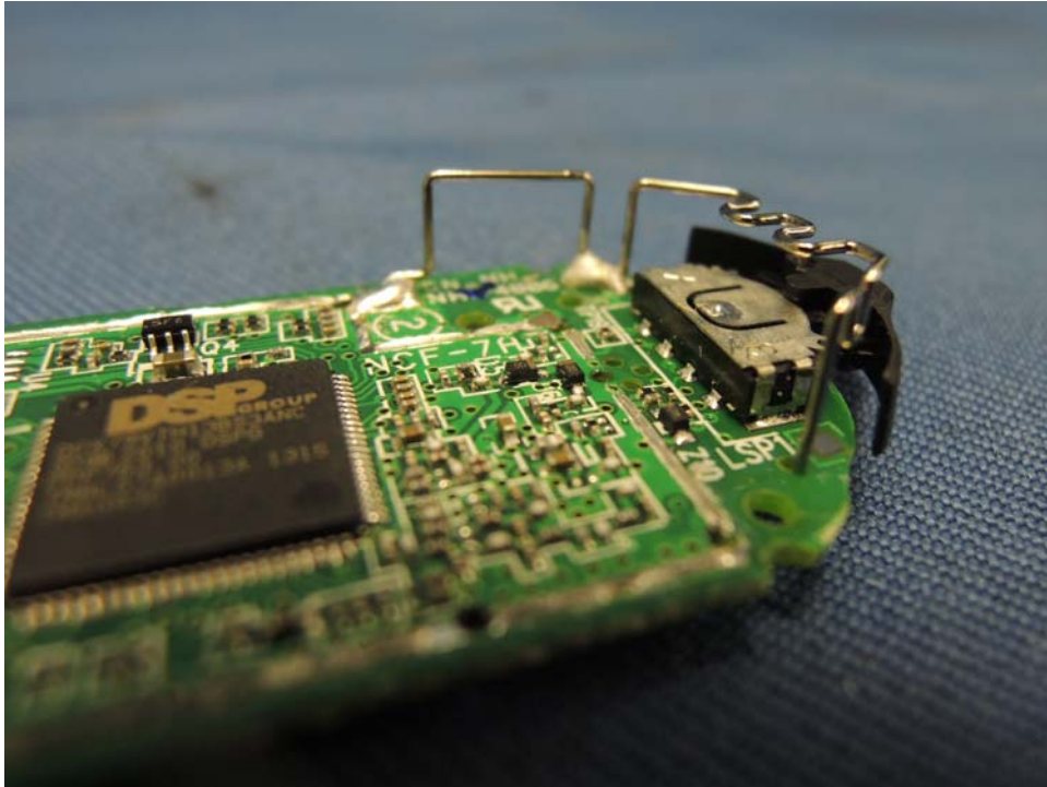
Headset Antenna (View 2)
