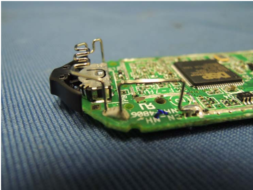
Headset Antenna (View 1)
