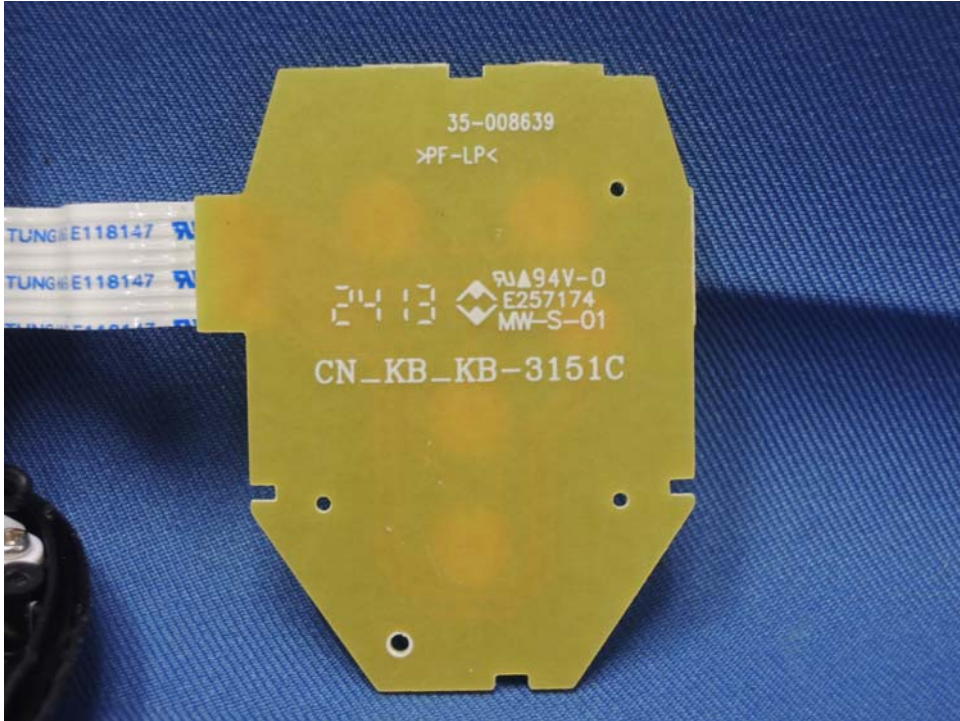
Speaker Keypad rear side
