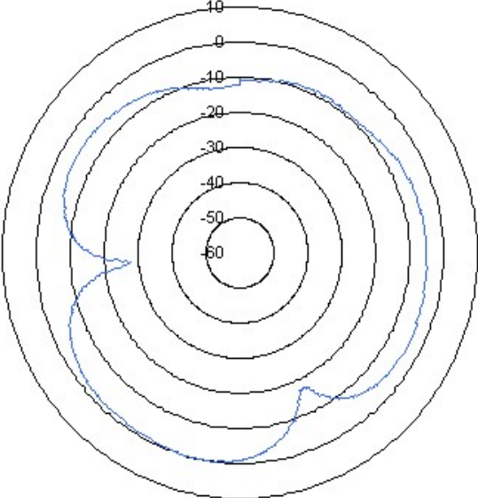
Antenna Gain
