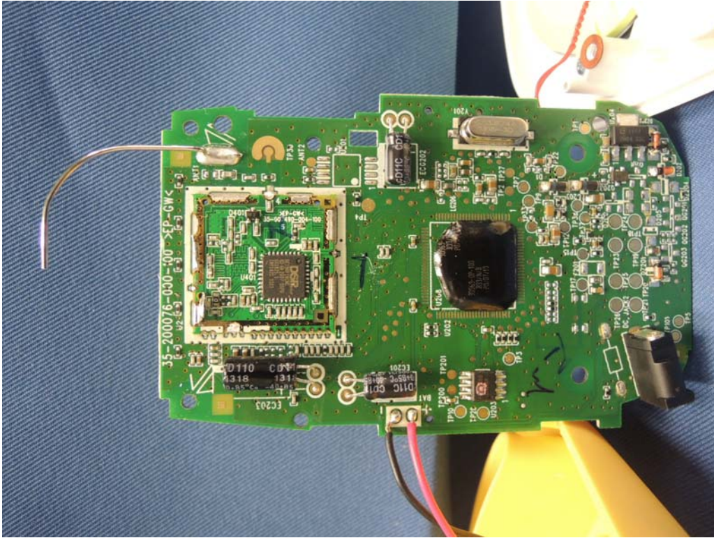
Parent Unit Main PCB comp side (View 2)
