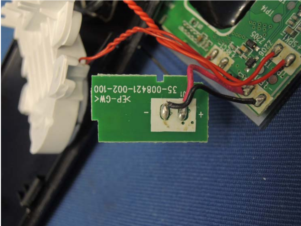
Handset Volume Board front side
