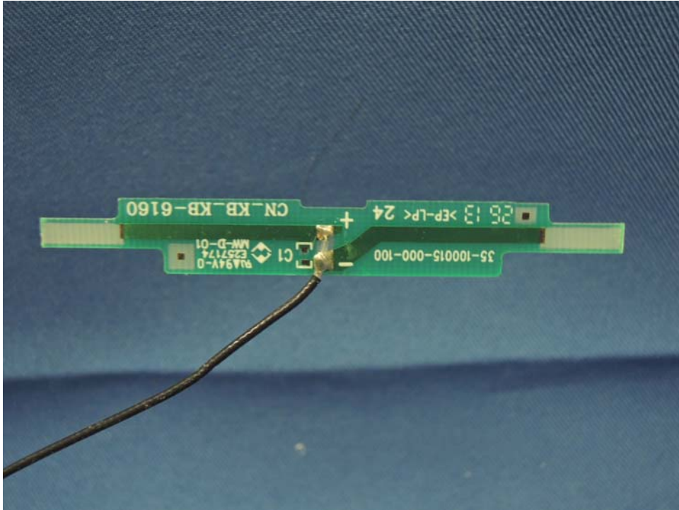
Base Unit BT Antenna (View 1)
