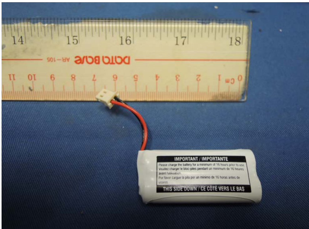
Figure 8 – 300mAh Coslight battery back view
