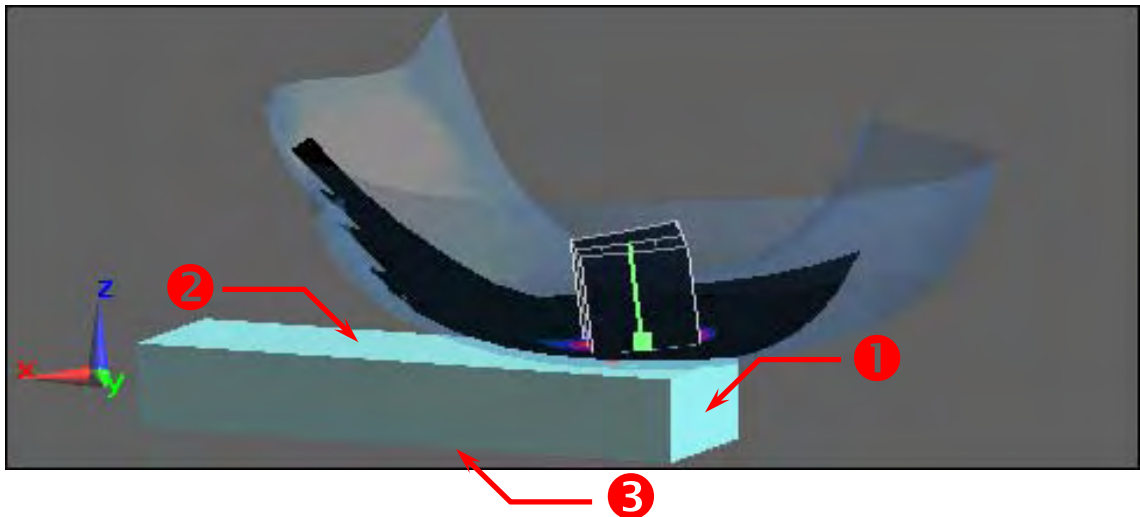
Figure 4. Left Head SAR Test Setup (Cheek)
