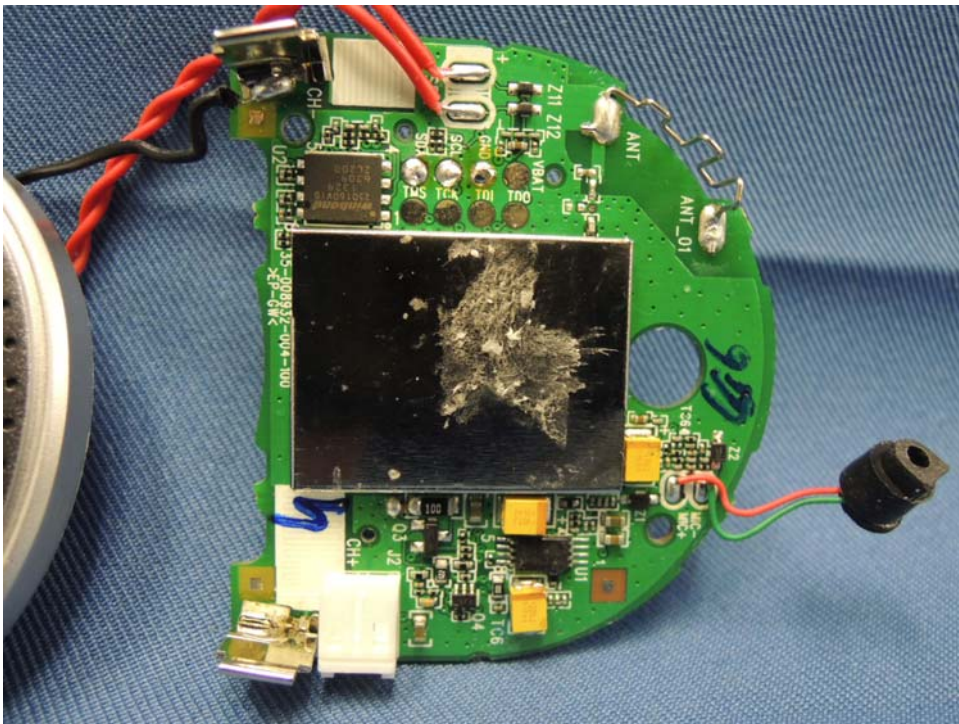
Speaker Main PCB comp side
