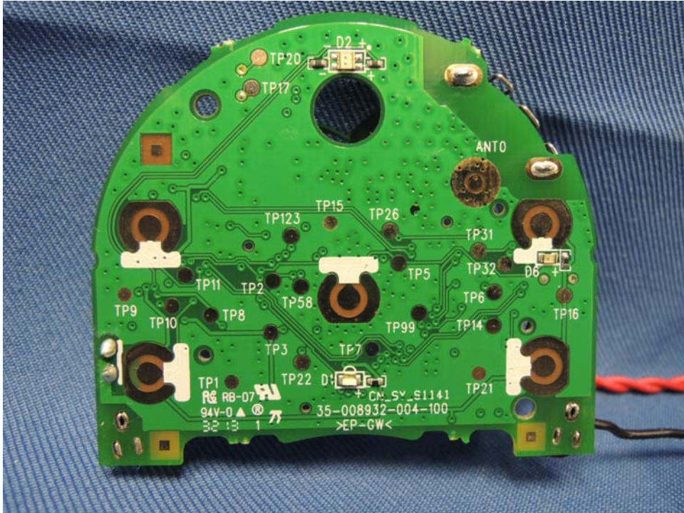
Speaker Main PCB solder side
