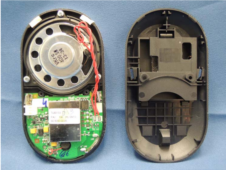
Speaker assembly
