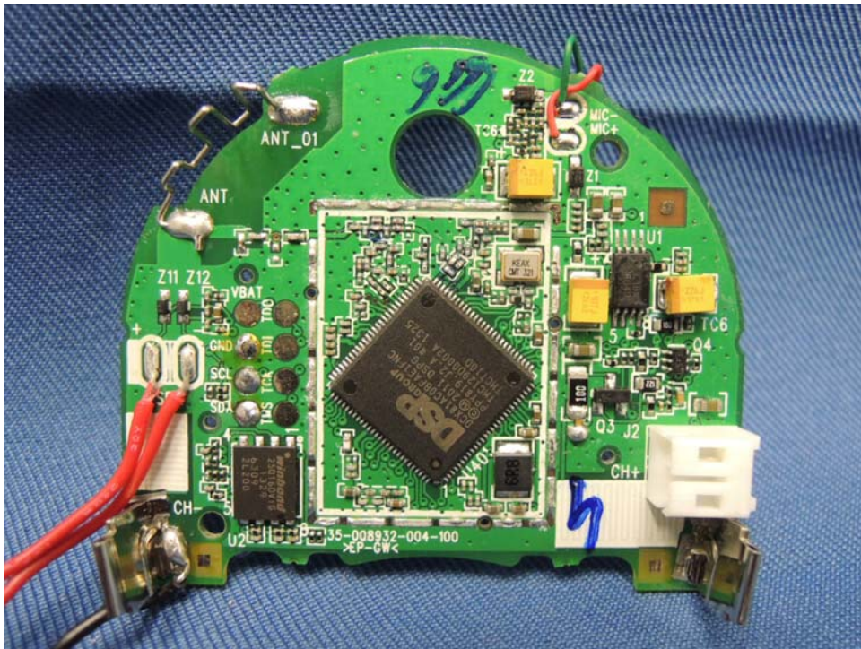
Speaker Oscillator PCB comp side
