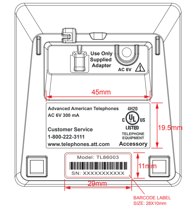
TL86003 Charger
