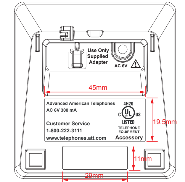
TL86103 Charger
