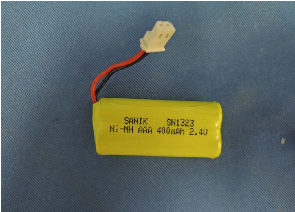
Figure 9 – 2.4VDC 400mAh Sanik battery front view
