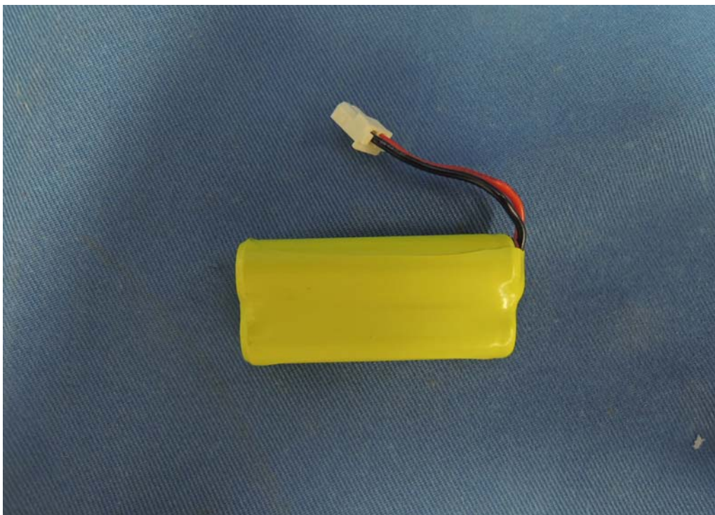
Figure 10 – 2.4VDC 400mAh Sanik battery back view
