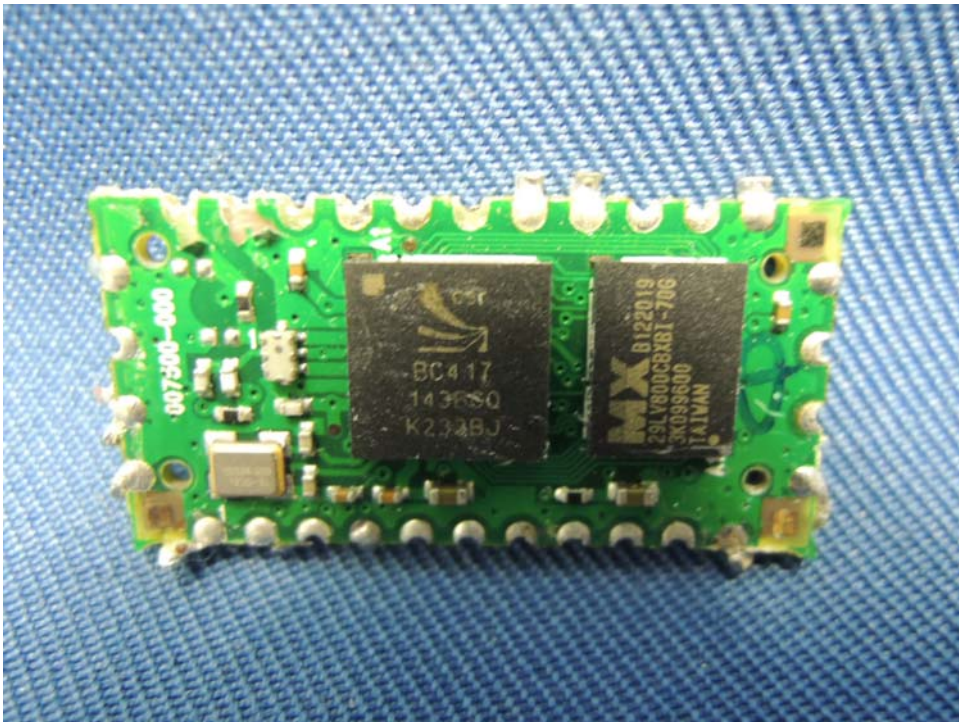
Base Unit Bluetooth Module PCB comp side
