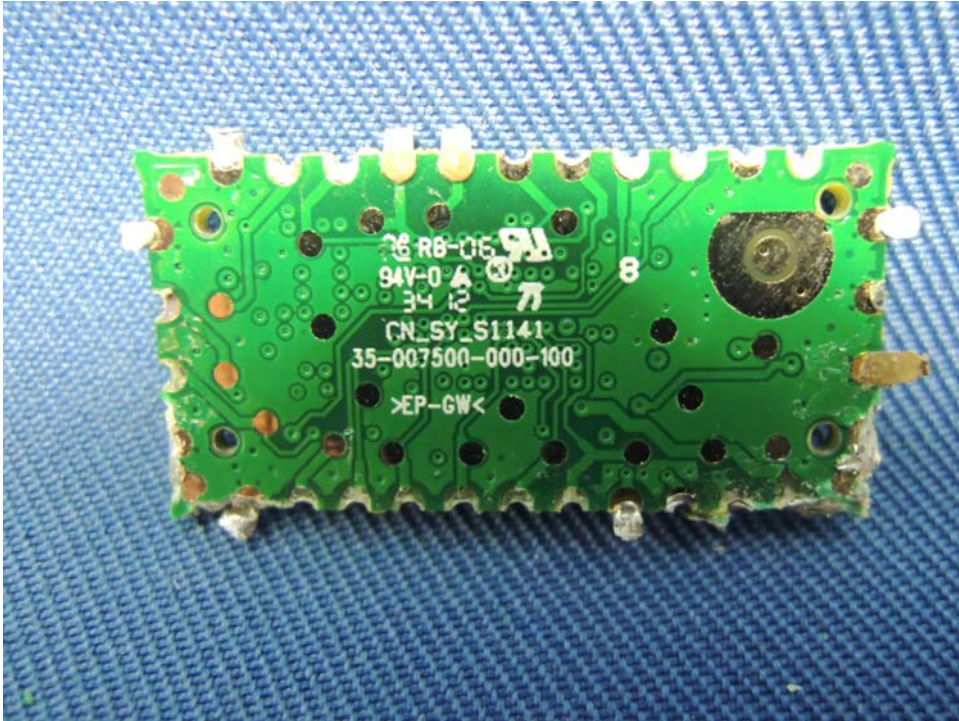
Base Unit Bluetooth Module PCB solder side
