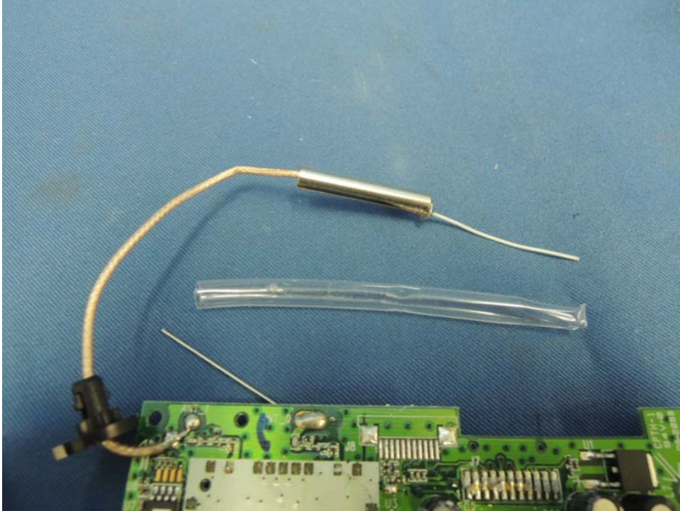
Base Unit DECT Antenna (ANT1)
