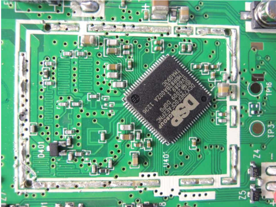
Handset DECT Module PCB comp side
