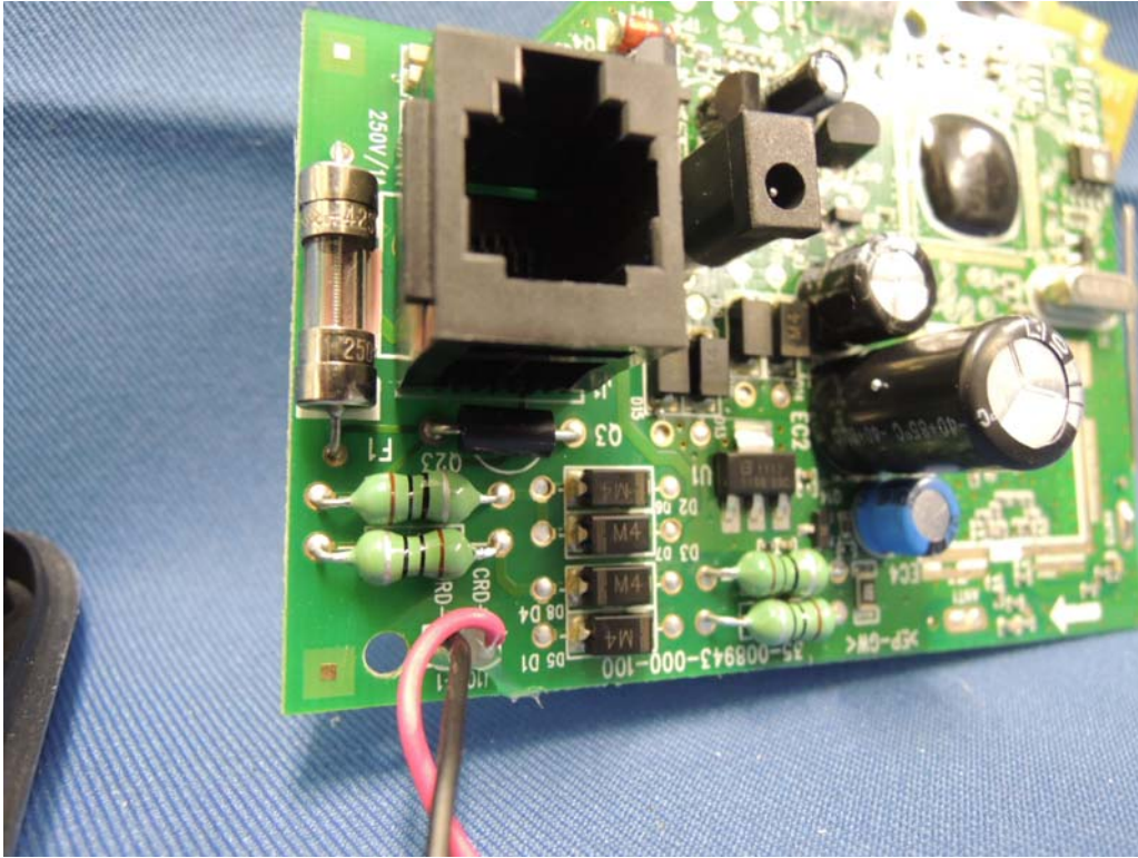
Base Unit Main PCB comp side (View 2)
