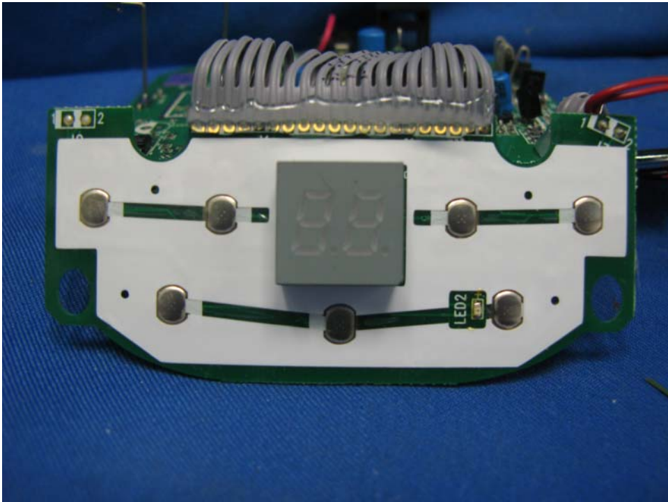
Base Unit DAM PCB front side
