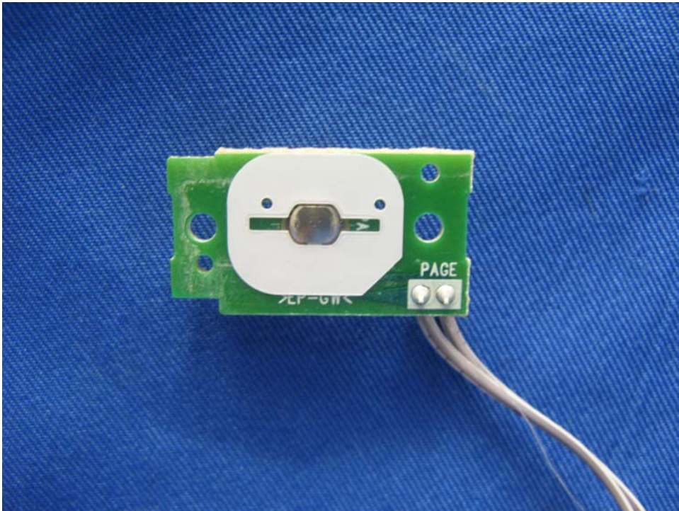
Base Unit Page Key PCB front side
