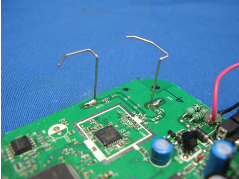
Base Unit Antennas
