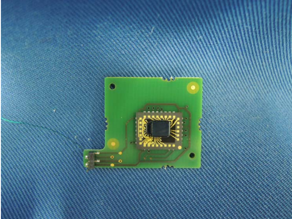
Handset Widex module PCB rear side
