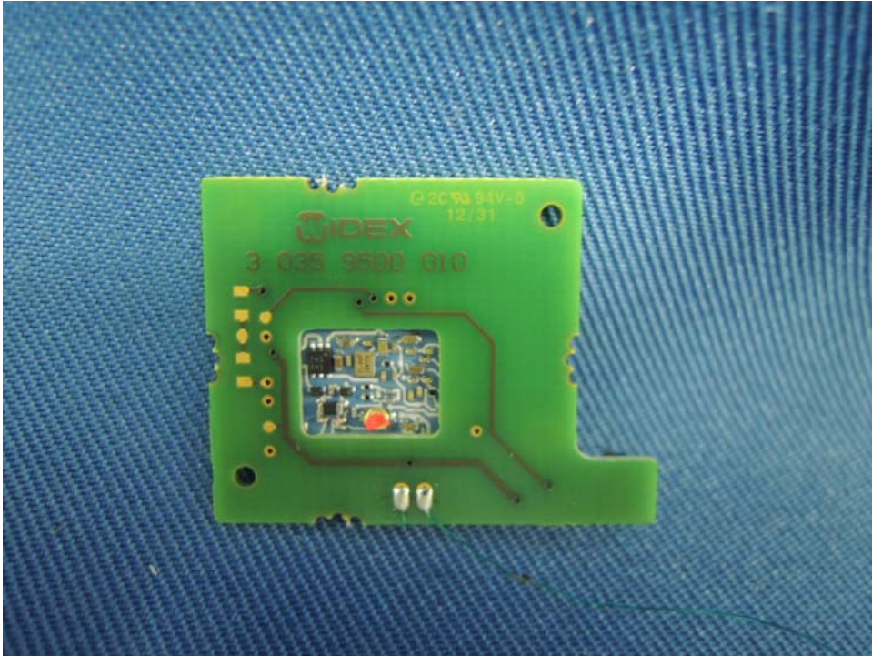
Handset Widex module PCB front side (View 1)
