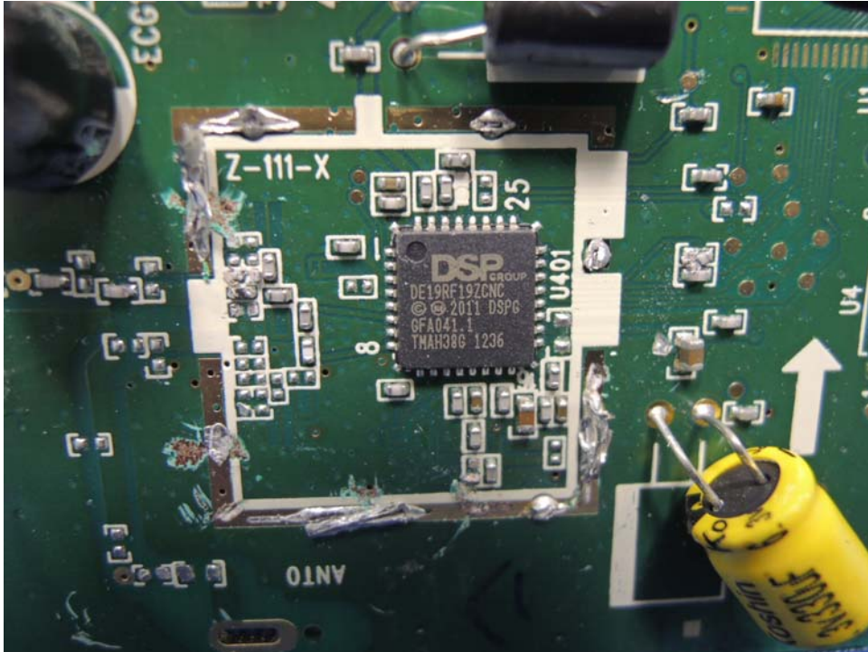
Base Unit DECT module PCB comp side
