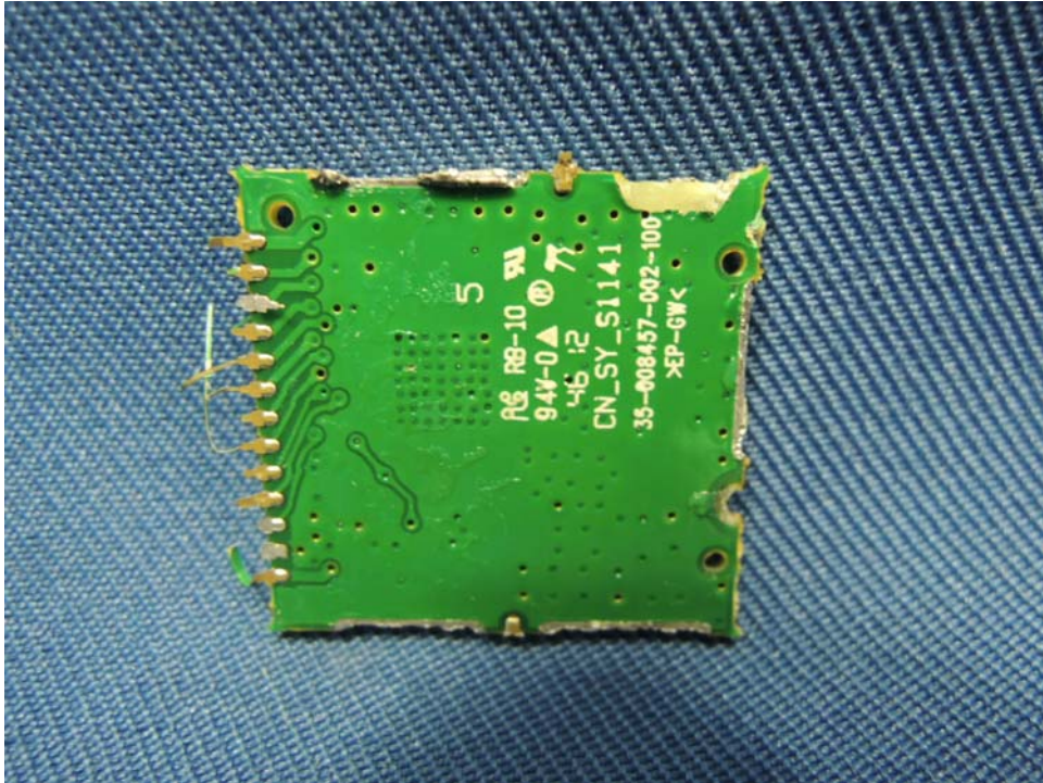
Handset DECT module PCB solder side
