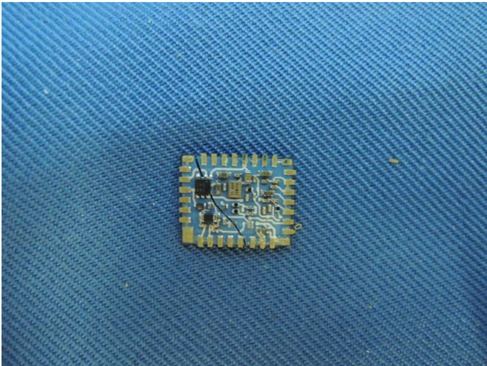
Handset Widex module PCB front side (View 2)
