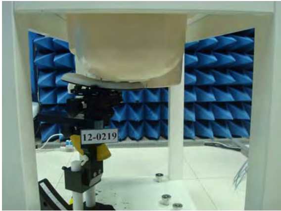
Figure 4. Left Head SAR Test Setup (Cheek)
