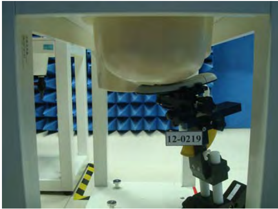
Figure 2. Right Head SAR Test Setup (Cheek)
