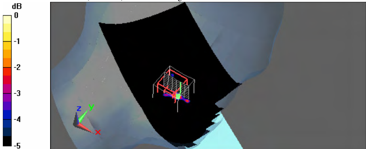
0 dB = 0.00455mW/g
