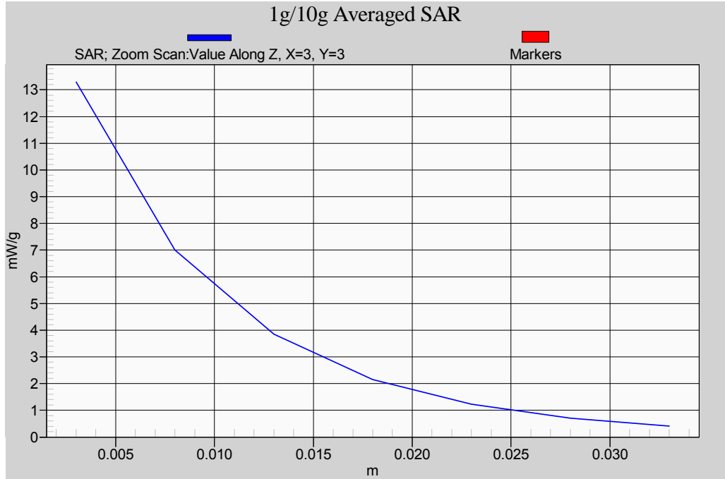
Head-Tissue-Simulating-Liquid 1950MHz
