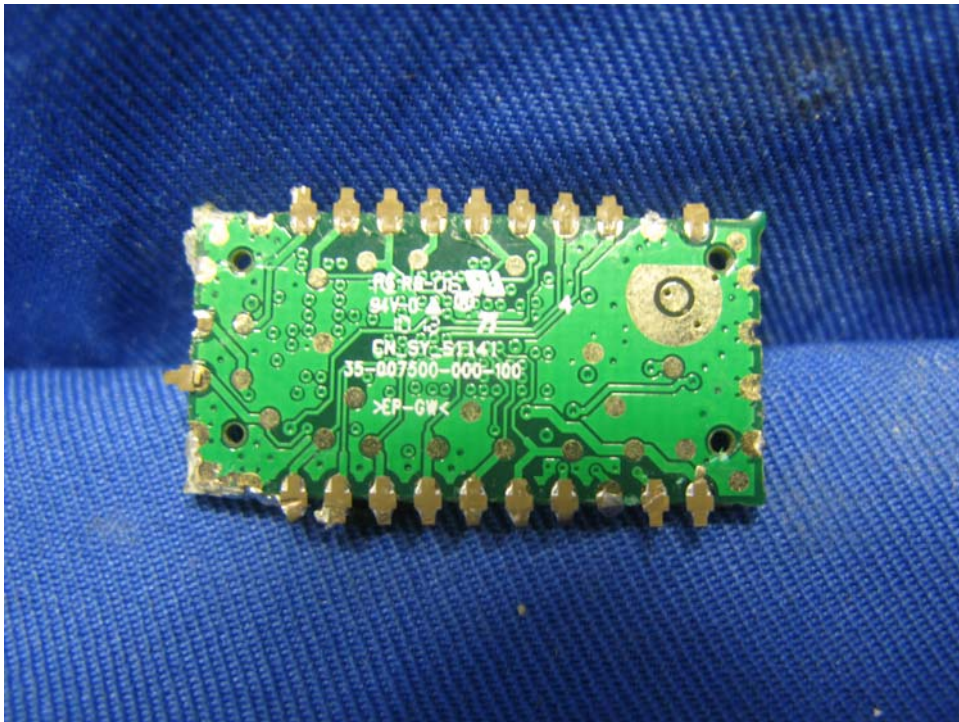
Base Unit Bluetooth RF Module PCB solder side comp side
