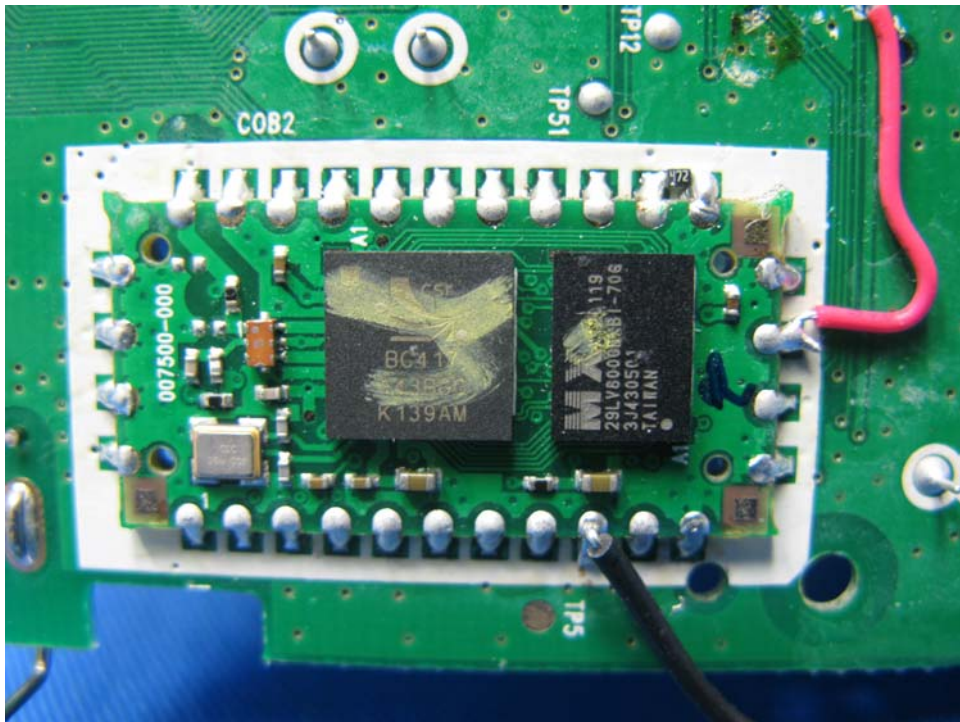
Base Unit Bluetooth RF Module PCB comp side view (1)
