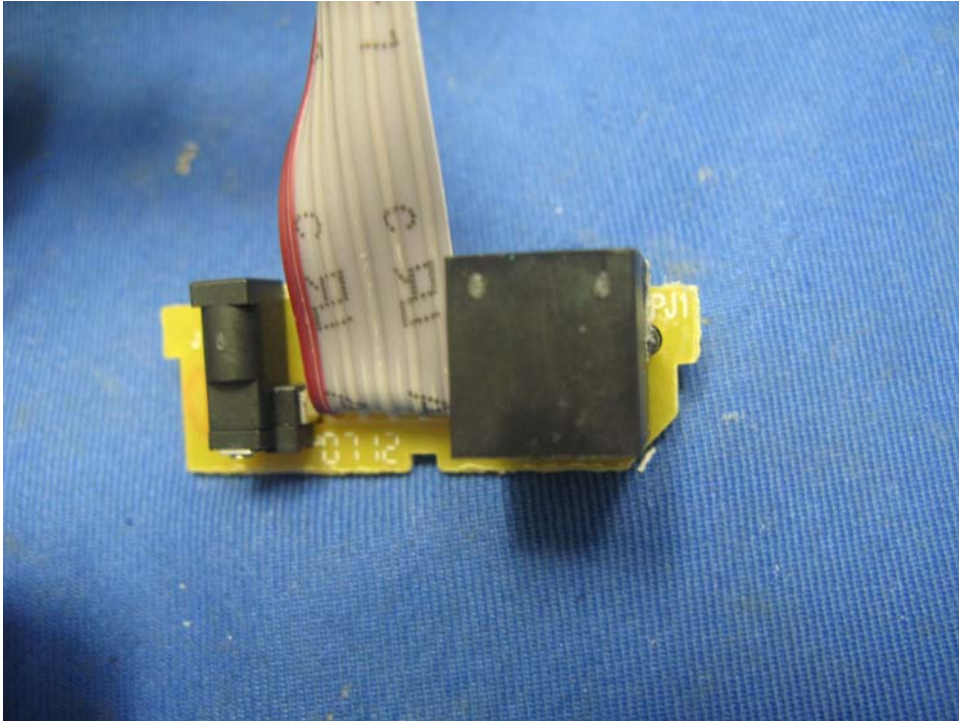
Base Unit Telephone Line & AC Jack Board front side (View 2)
