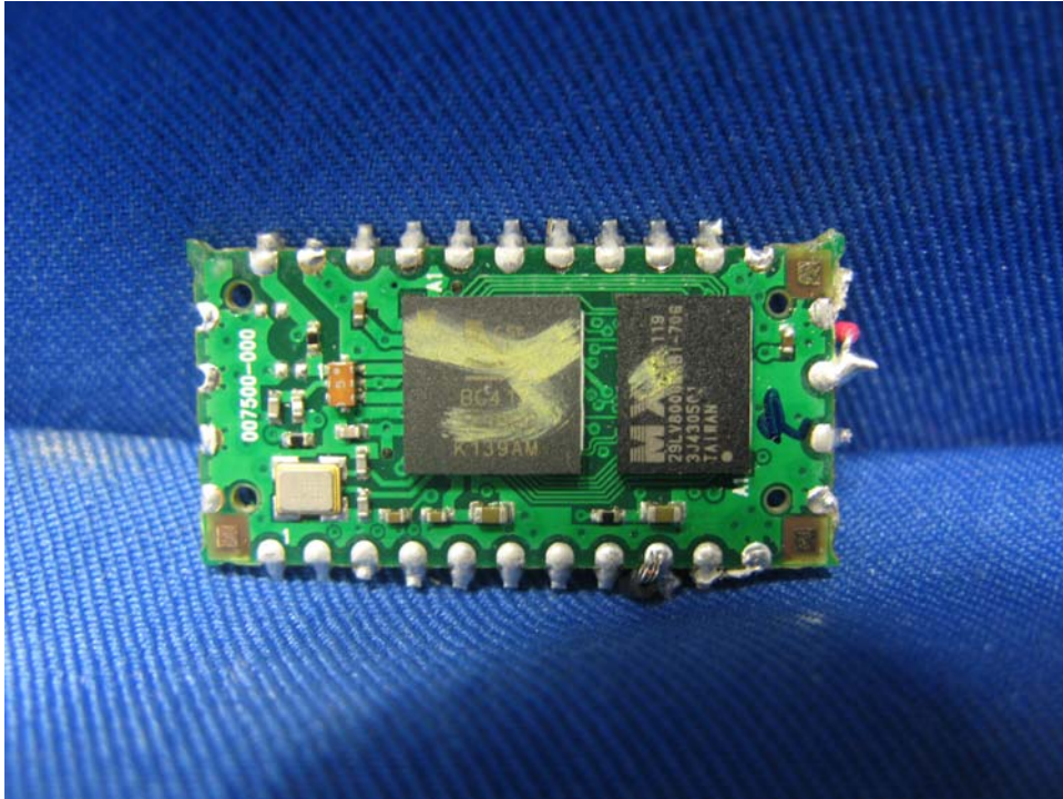
Base Unit Bluetooth RF Module PCB comp side view (2)
