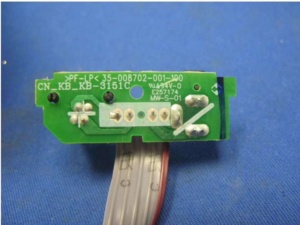
Base Unit Telephone Line & AC Jack Board rear side
