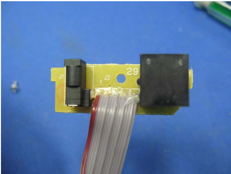
Base Unit Telephone Line & AC Jack Board front side (View 1)
