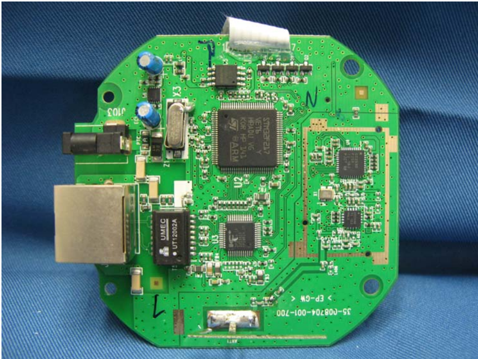
Zigbee IP Bridge Main PCB comp side
