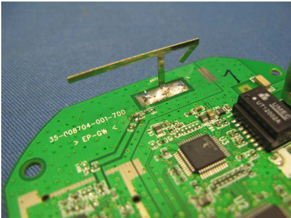
Zigbee IP Bridge Antenna
