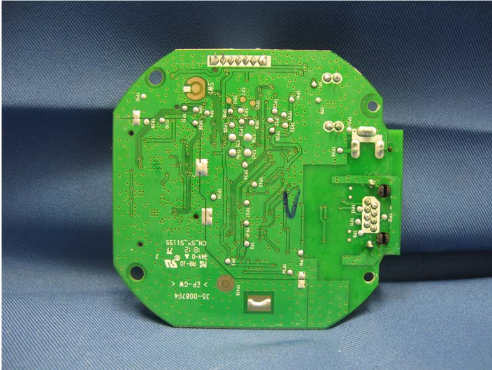
Zigbee IP Bridge Main PCB solder side
