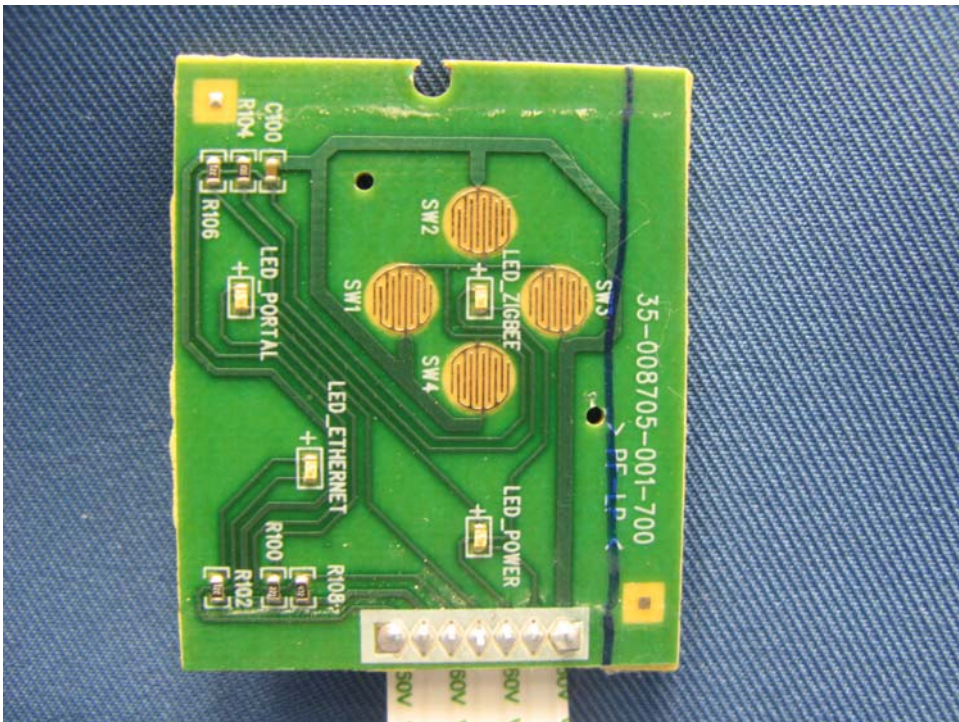
Zigbee IP Bridge Keypad front side
