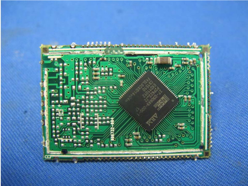
Base Unit RF Slave PCB comp side
