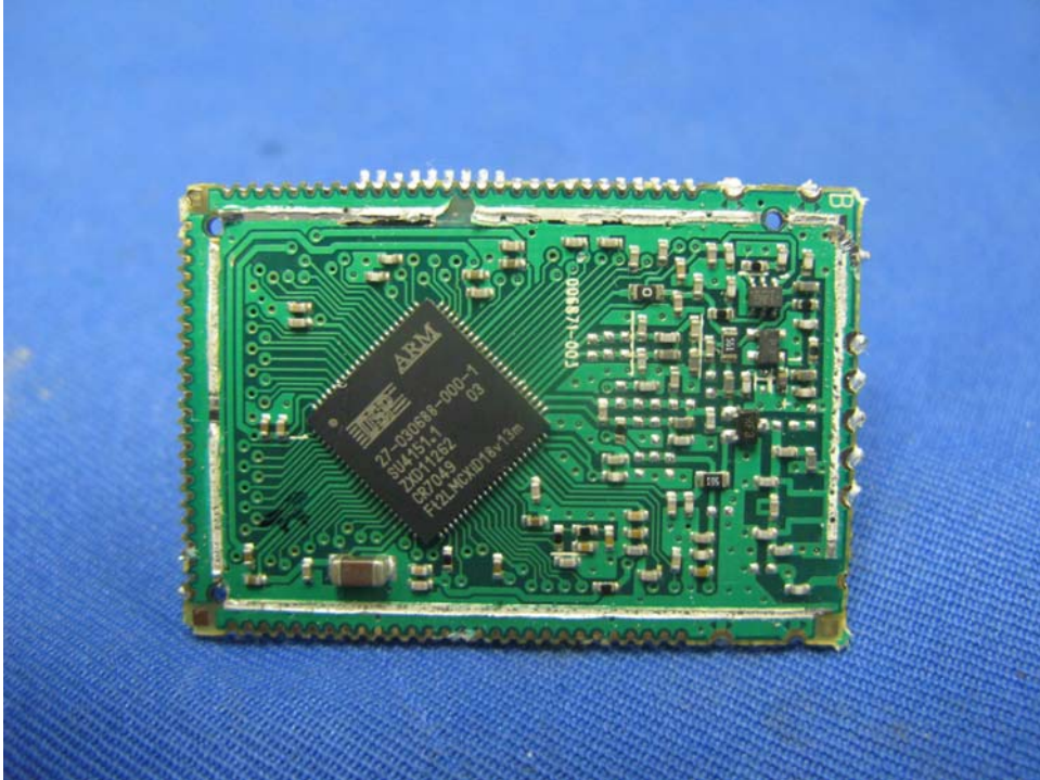
Base Unit RF Master PCB comp side
