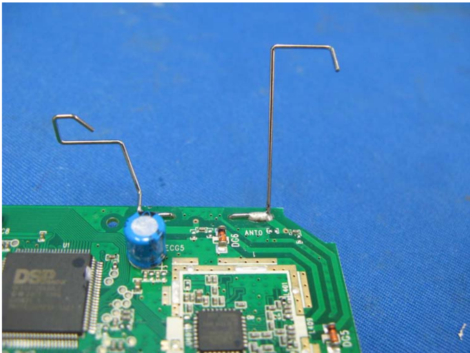
Base Unit DECT Antennas
