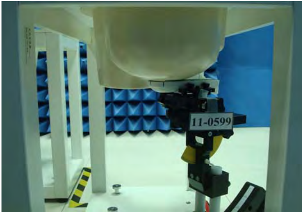
Figure 2. Right Head SAR Test Setup (Cheek)
