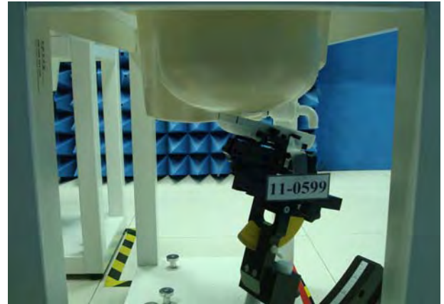
Figure 3. Right Head SAR Test Setup (Tilted)
