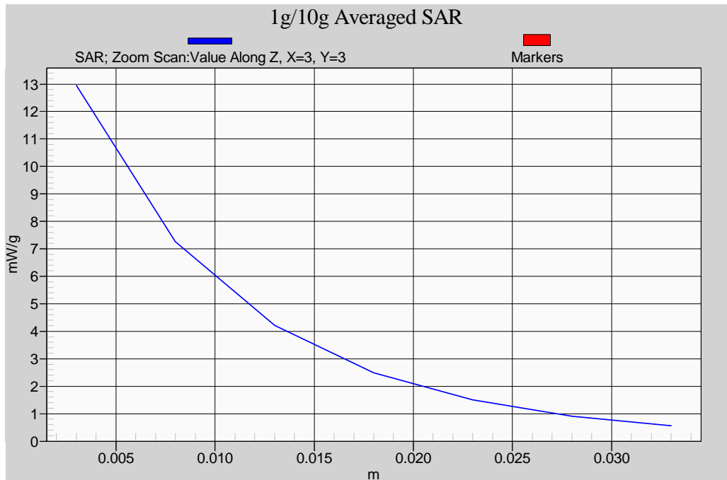
Body-Tissue-Simulating-Liquid 1900MHz
