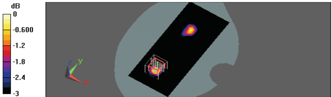
0 dB = 0.018mW/g
