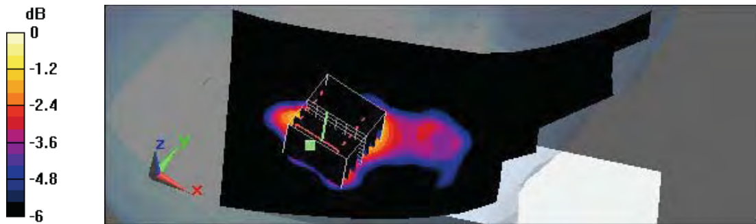
0 dB = 0.013mW/g
