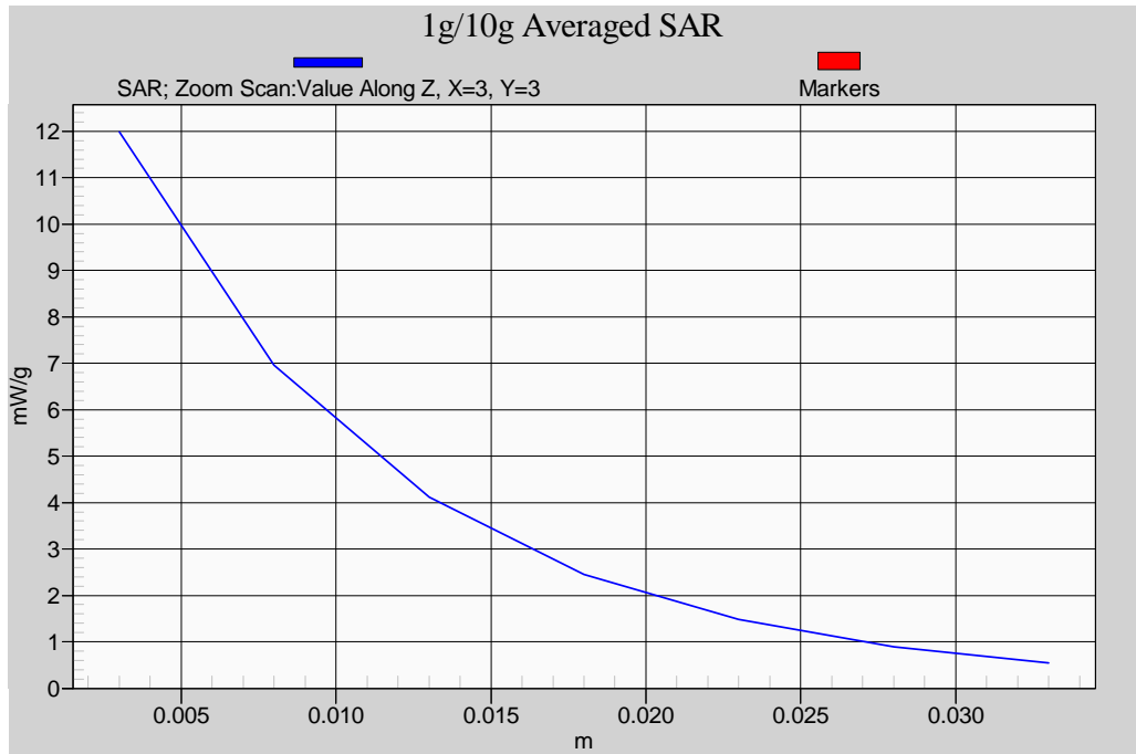
Head-Tissue-Simulating-Liquid 1900MHz
